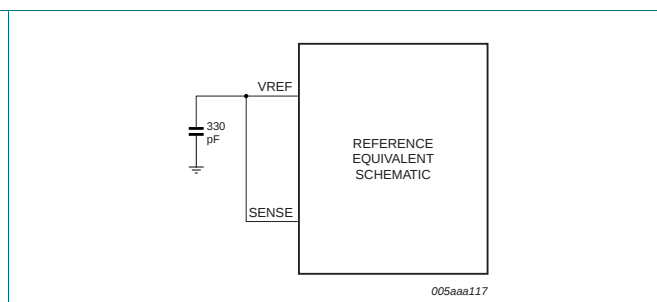
Fig 12. Internal reference, 1 V (p-p) full-scale
