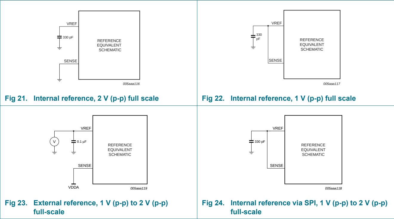
Figure 21 to Figure 24 illustrate how to connect the SENSE and VREF pins to select the required reference voltage source.
