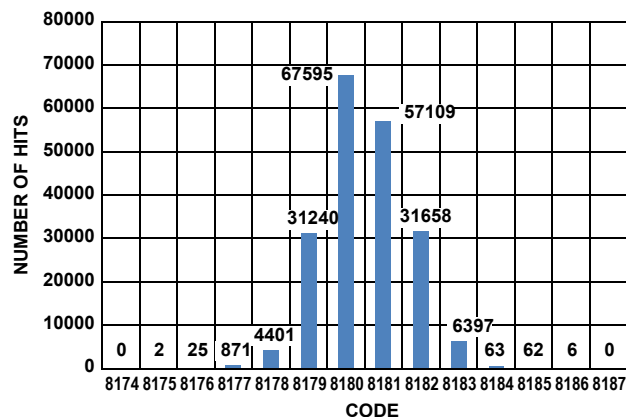
FIGURE 15. NOISE HISTOGRAM
