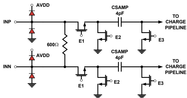
FIGURE 45. ANALOG INPUTS
