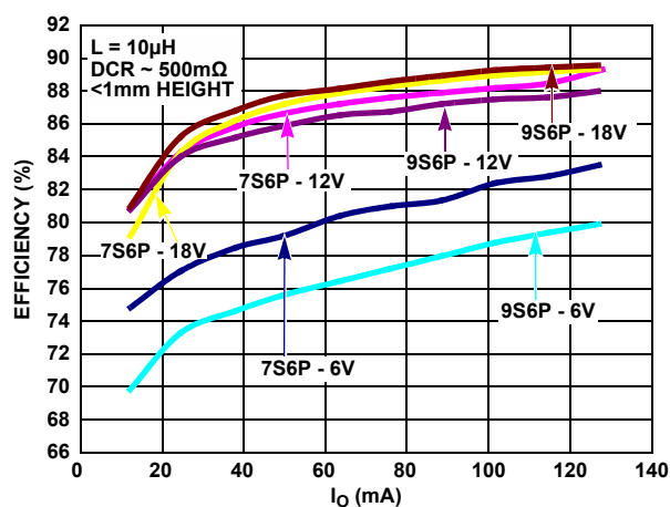
FIGURE 5. 3 EFFICIENCY, L = 10\mu\text{H} WITH \text{DCR} = 500\text{m}\Omega , 1\text{mm} , C_O = 4 \times 4.7\mu\text{F}/50\text{V}
