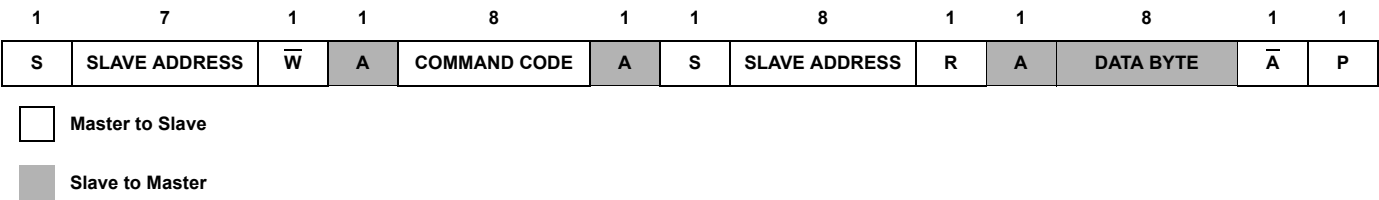
FIGURE 32. READ BYTE PROTOCOL
