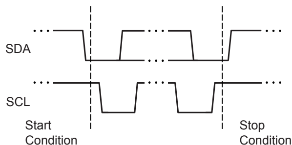
(A) Start and Stop Conditions
