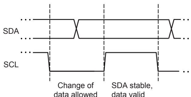
(B) Clock and Data Bit Synchronization
