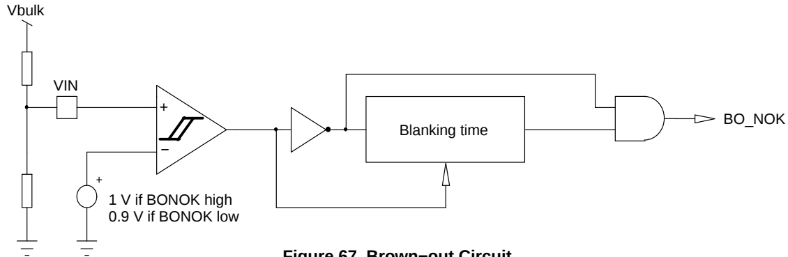
Figure 67. Brown-out Circuit
