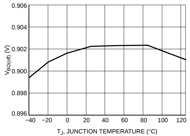
Figure 44. V BO(off) vs. Junction Temperature
