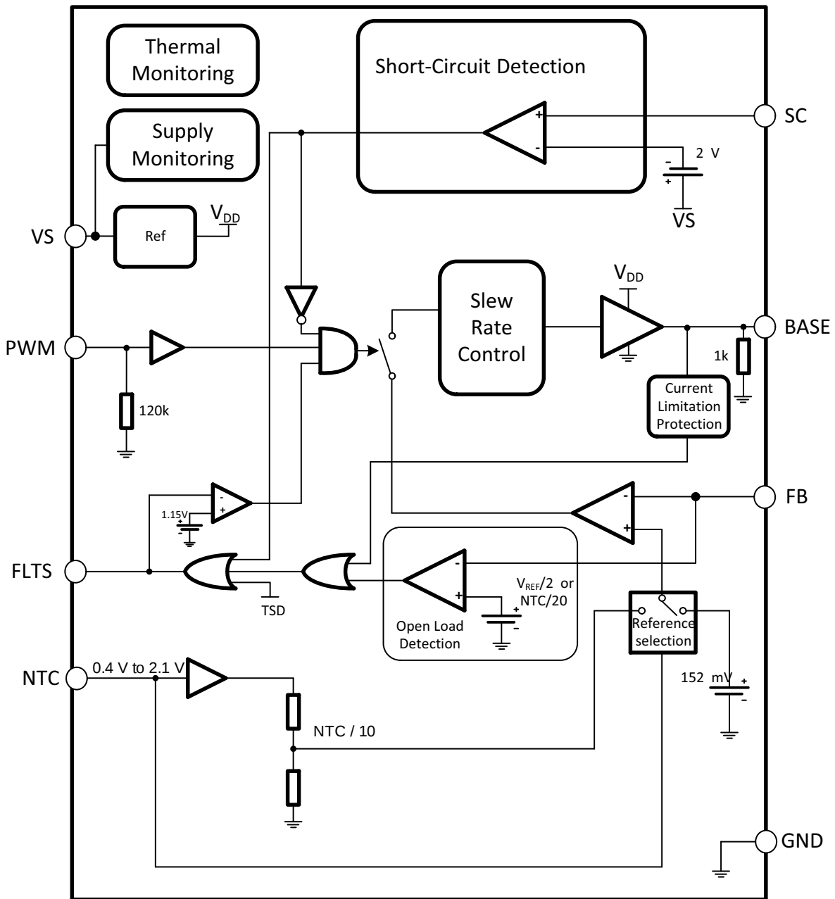
Figure 3. Block Diagram
