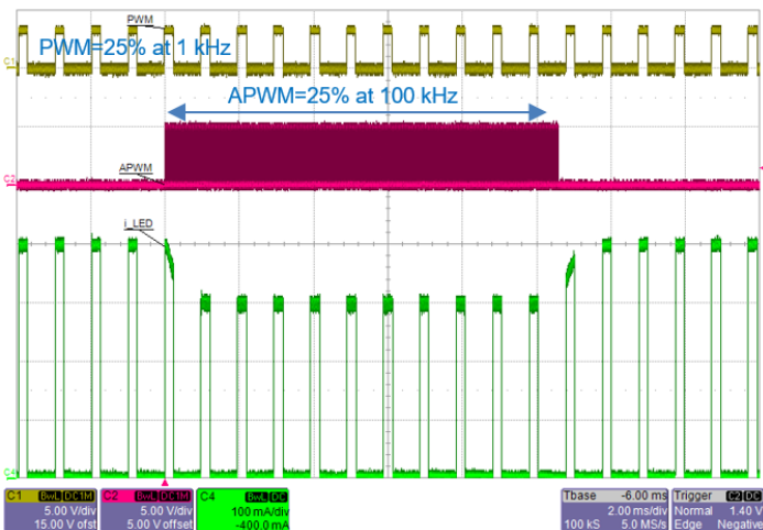
Figure 29: PWM = 25% at 1 kHz. Peak LED current drops from 400 mA ( 4 \times 100 mA/ch) to 300 mA when APWM of 25% duty cycle is applied
