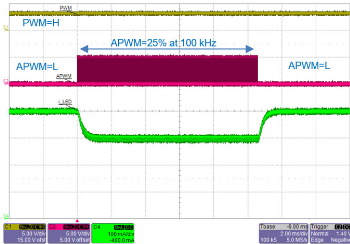
Figure 28: PWM = H. Total LED current drops from 400 mA ( 4 \times 100 mA/ch) to 300 mA when APWM of 25% duty cycle is applied. Note that LED current takes \sim 0.5 ms to settle after change in APWM.
