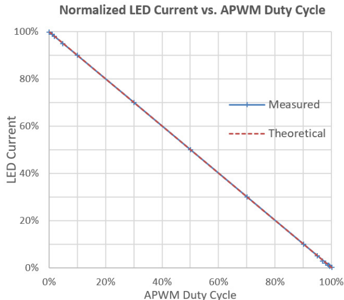
Figure 30: Showing LED current is inversely proportional to the APWM duty cycle. Test conditions: V_{IN} = 12\text{ V} , V_{OUT} = 25\text{ V} ( 8 \times \text{WLED} ), total LED current = 100\text{ mA} \times 4 , APWM frequency = 100\text{ kHz}
