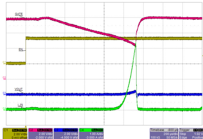
Figure 46: Startup into an output shorted-to-GND fault. Input OCP is tripped when current (Green trace) exceeds 4 A. PMOS Gate (Red) is turned off immediately and IC latches off.
