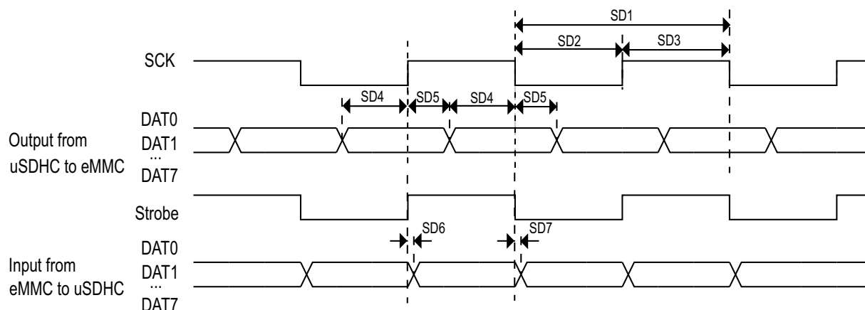
Figure 43. HS400 timing
