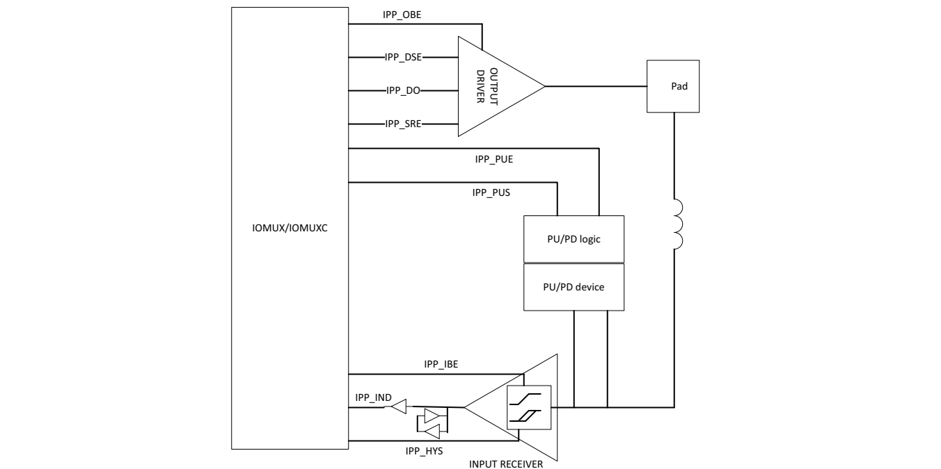
Figure 8. GPIO block diagram
