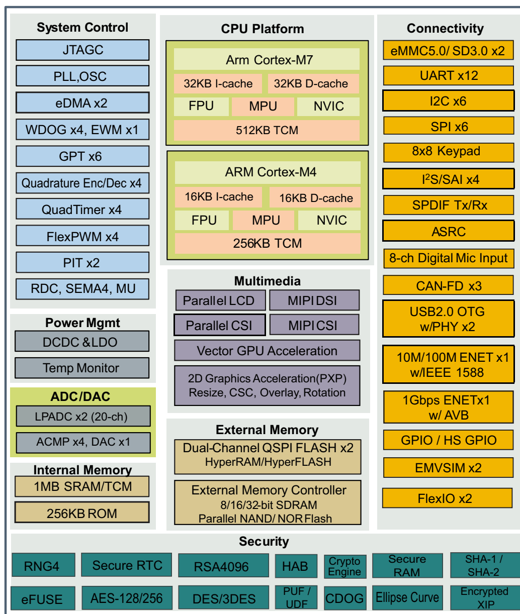
Figure 3. i.MX RT1160 system block diagram
