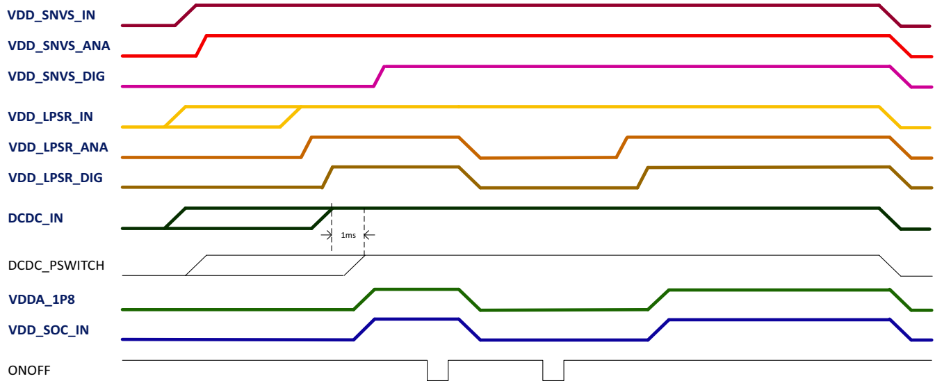
Figure 4. Power sequence
