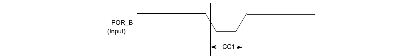
Figure 9. POR reset timing diagram
