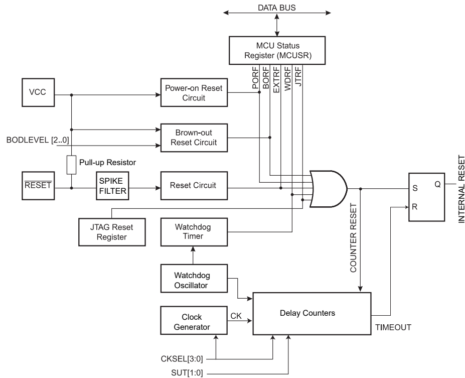
Figure 12-1. Reset Logic
