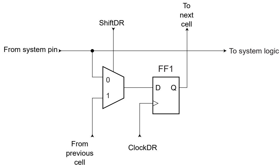
Figure 26-7. Observe-only Cell
