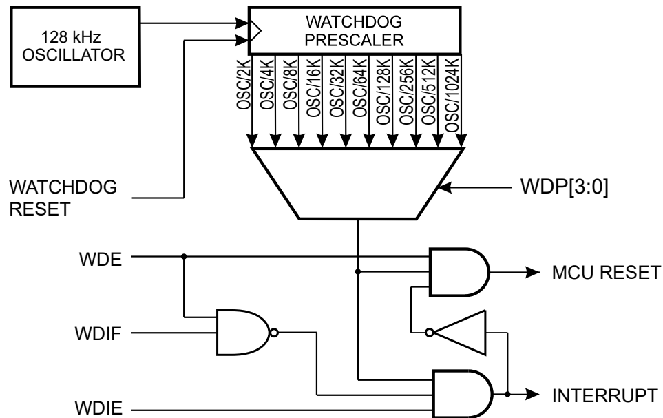
Figure 12-7. Watchdog Timer
