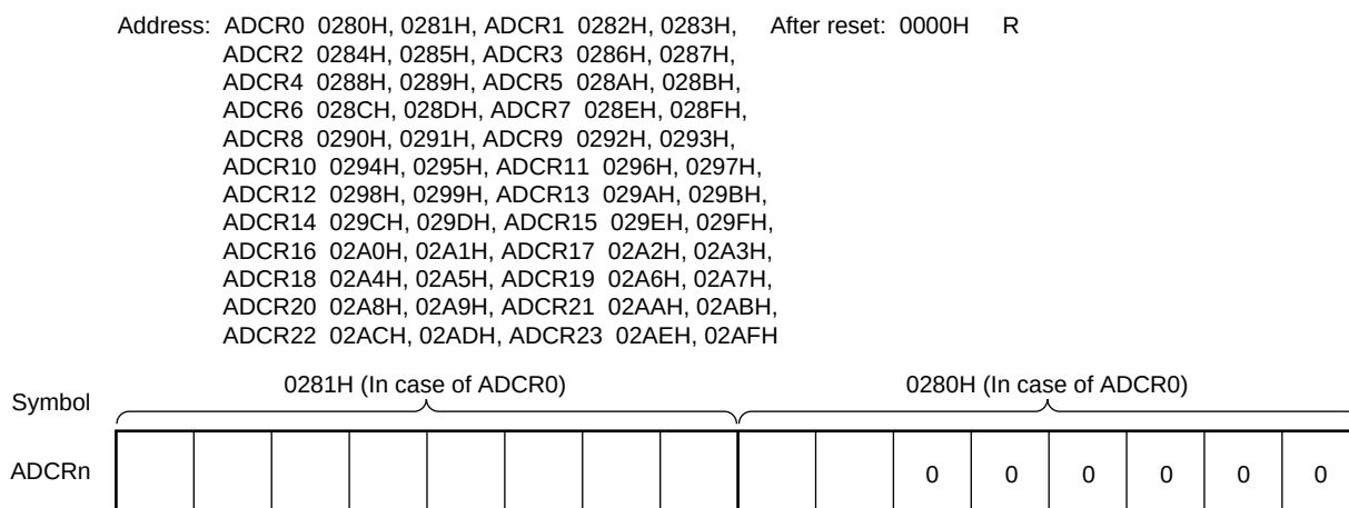
Figure 10-9. Format of 10-bit A/D Conversion Result Register n (ADCRn)
