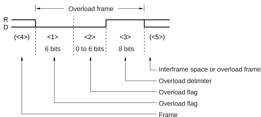
Figure 13-16. Overload Frame
