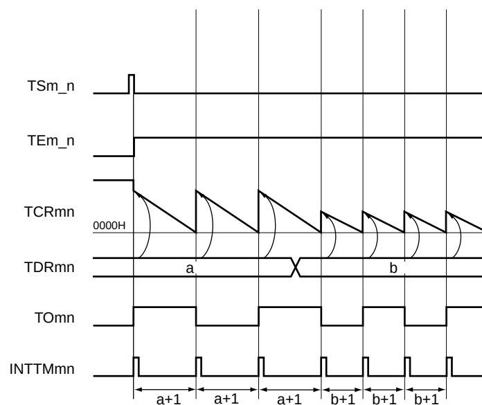
Figure 6-45. Example of Basic Timing of Operation as Interval Timer/Square Wave Output (MDmn0 = 1)
