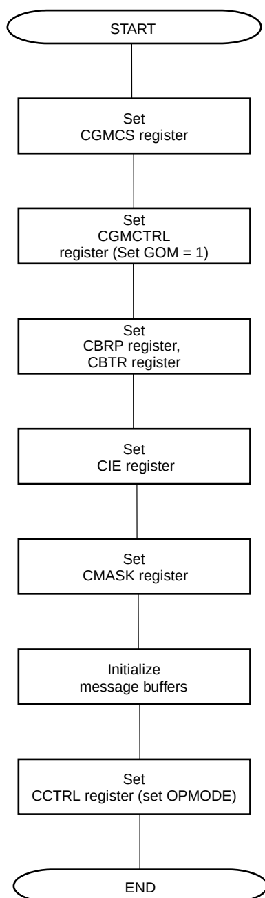
Figure 13-63. Initialization
