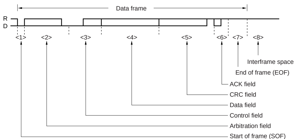
Figure 13-3. Data Frame
