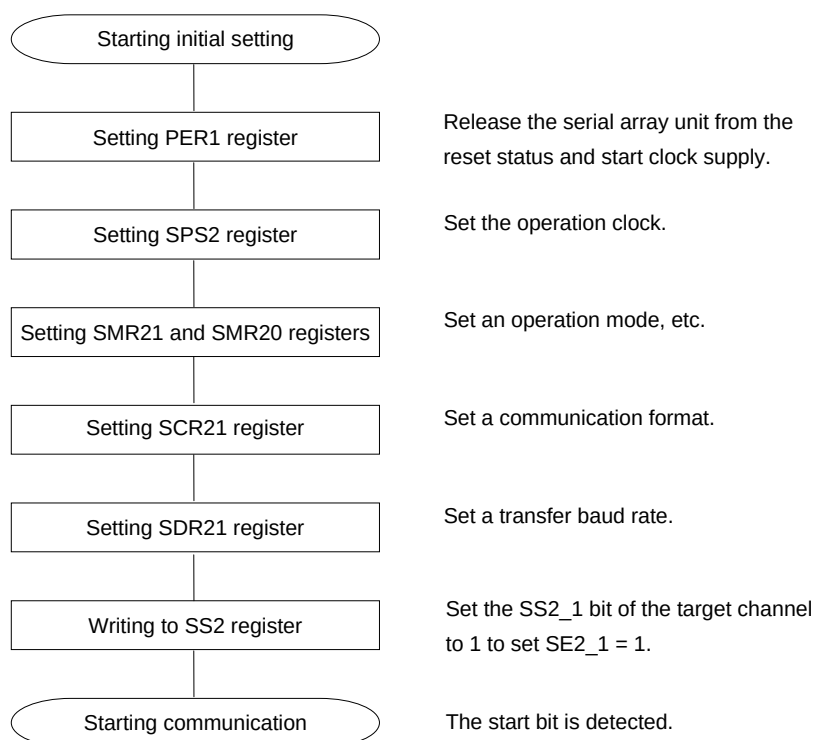
Figure 11-132. Initial Setting Procedure for UART Reception
