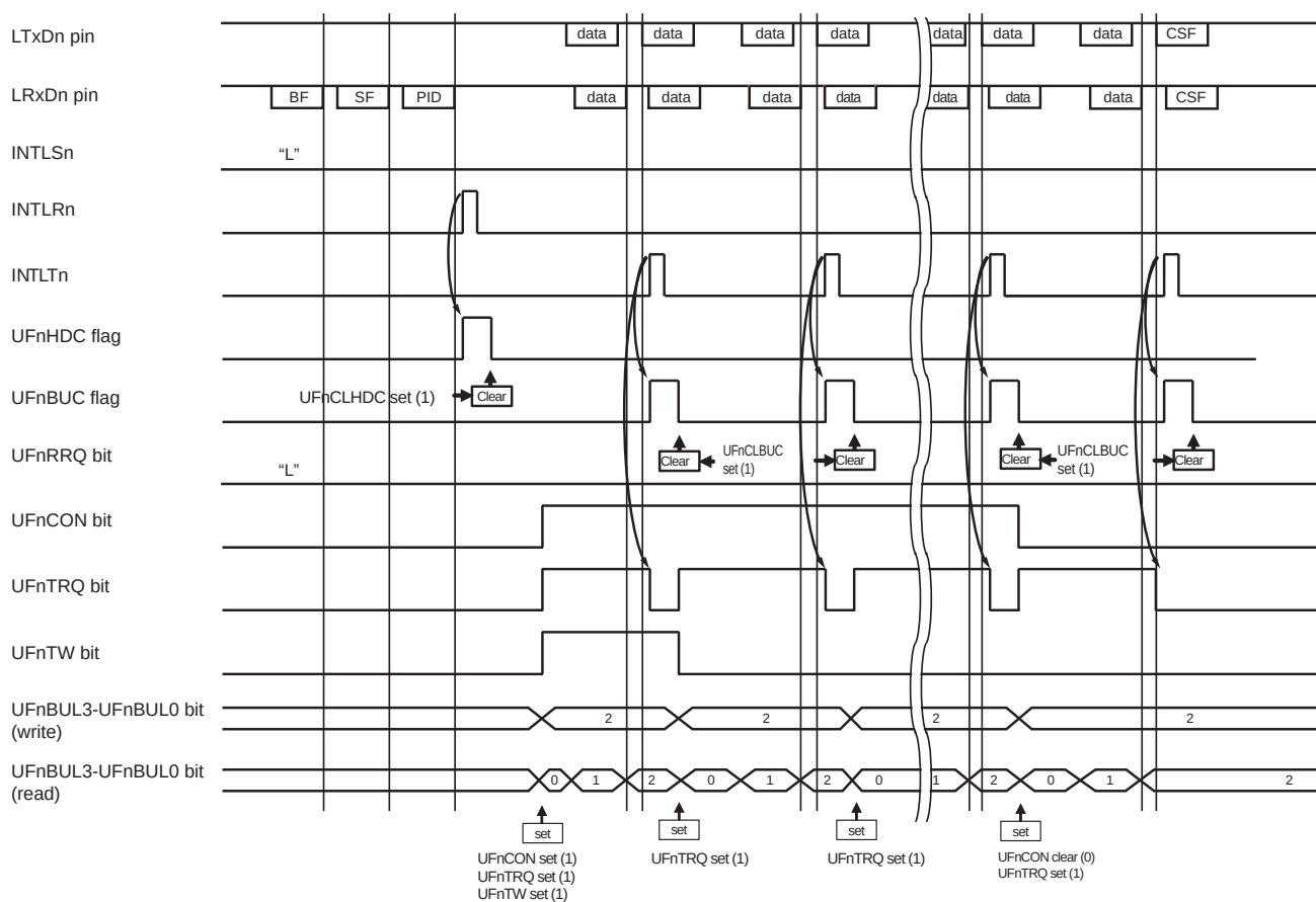
Figure 12-68. Multi-Byte Transmission Implementation Example
