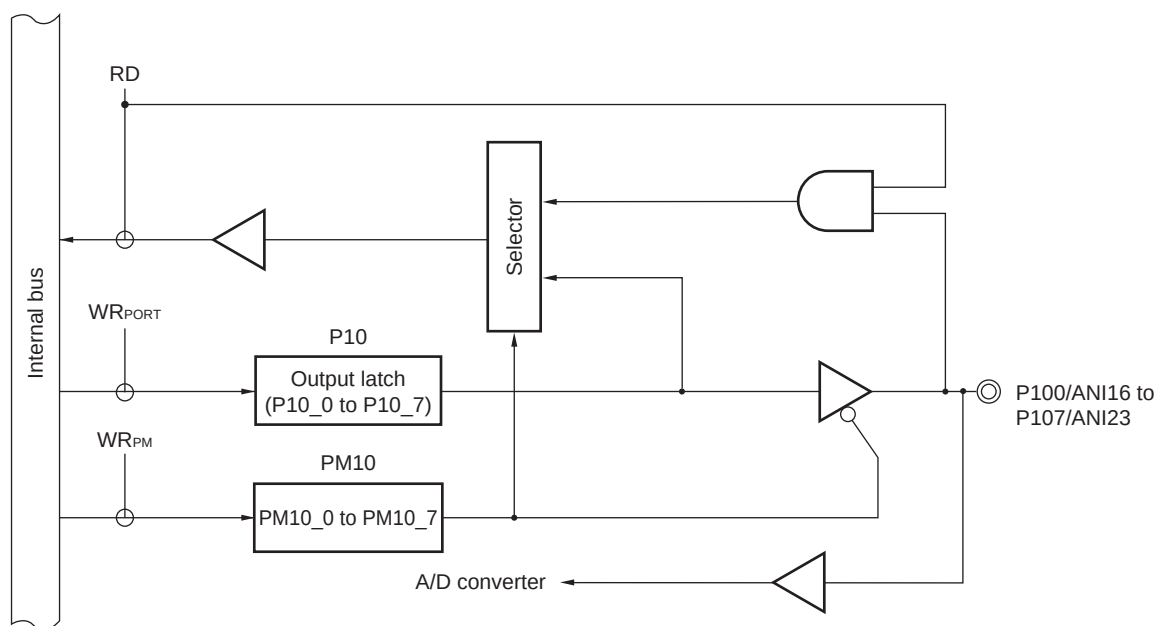
Figure 4-68. Block Diagram of P100 to P107
