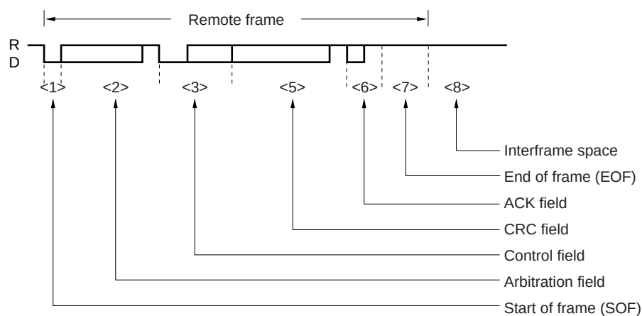
Figure 13-4. Remote Frame
