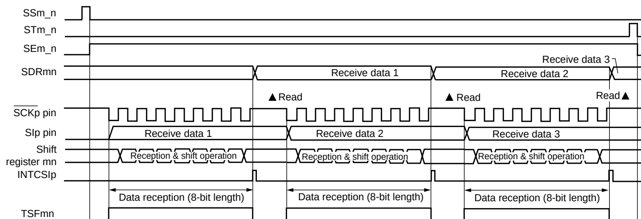
Figure 11-63. Timing Chart of Slave Reception (in Single-Reception Mode)
