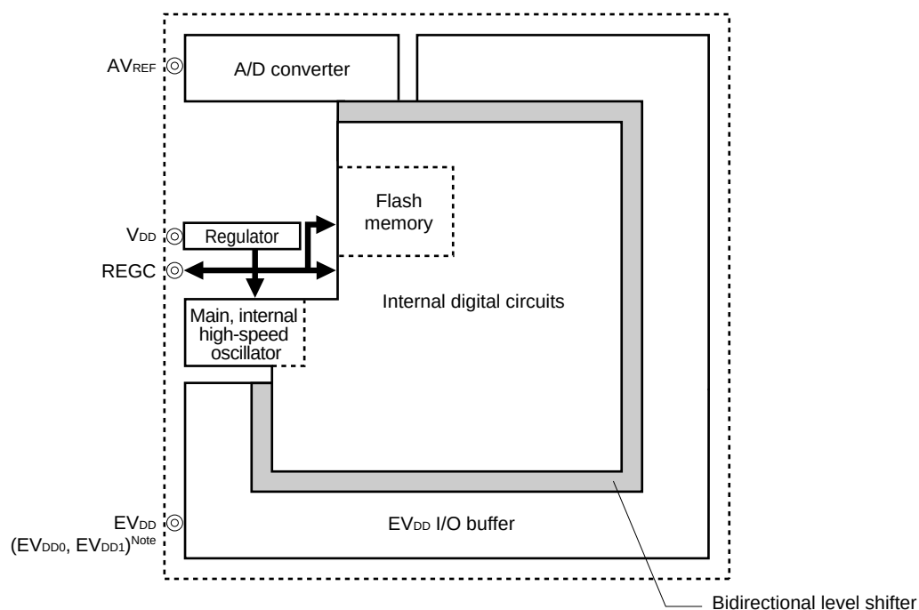
Figure 22-1. Regulator
