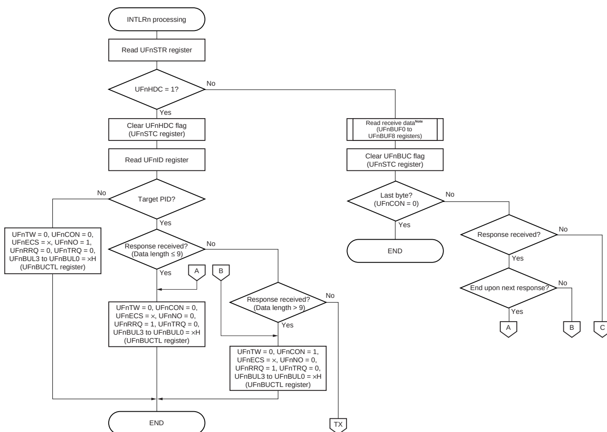
Figure 12-66. Multi-Byte Transmission/Reception Processing Flow Example (1/2)
