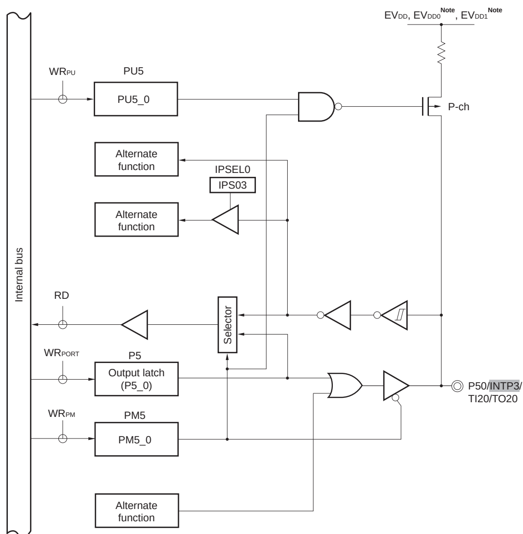
Figure 4-45. Block Diagram of P50
