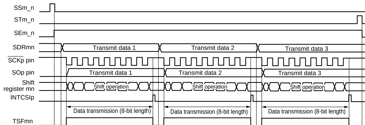
Figure 11-31. Timing Chart of Master Transmission (in Single-Transmission Mode) (Type 1: DAPmn = 0, CKPmn = 0)
