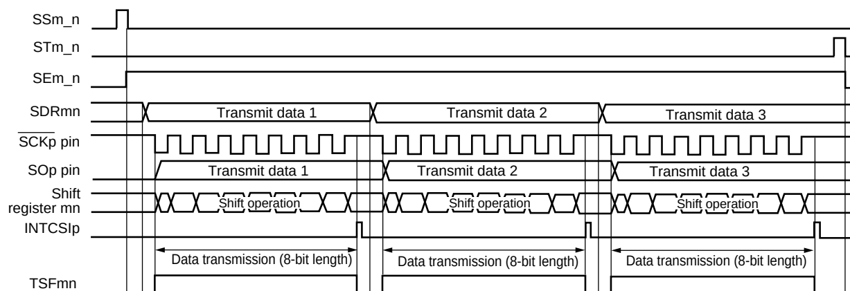
Figure 11-80. Timing Chart of Master Transmission (in Single-Transmission Mode) (Type 1: DAPmn = 0, CKPmn = 0)
