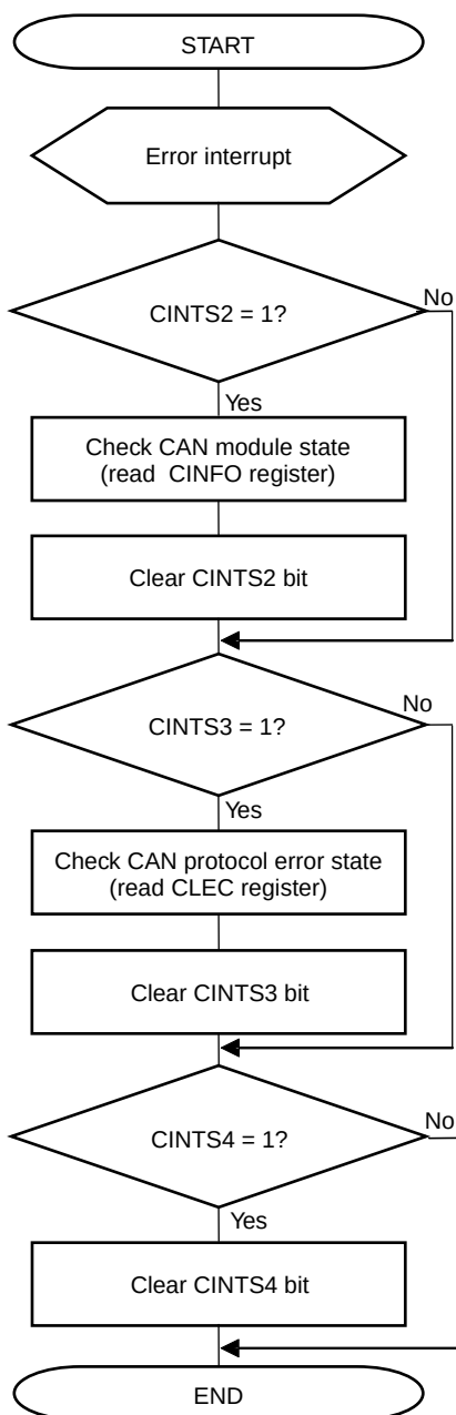
Figure 13-86. Error Handling
