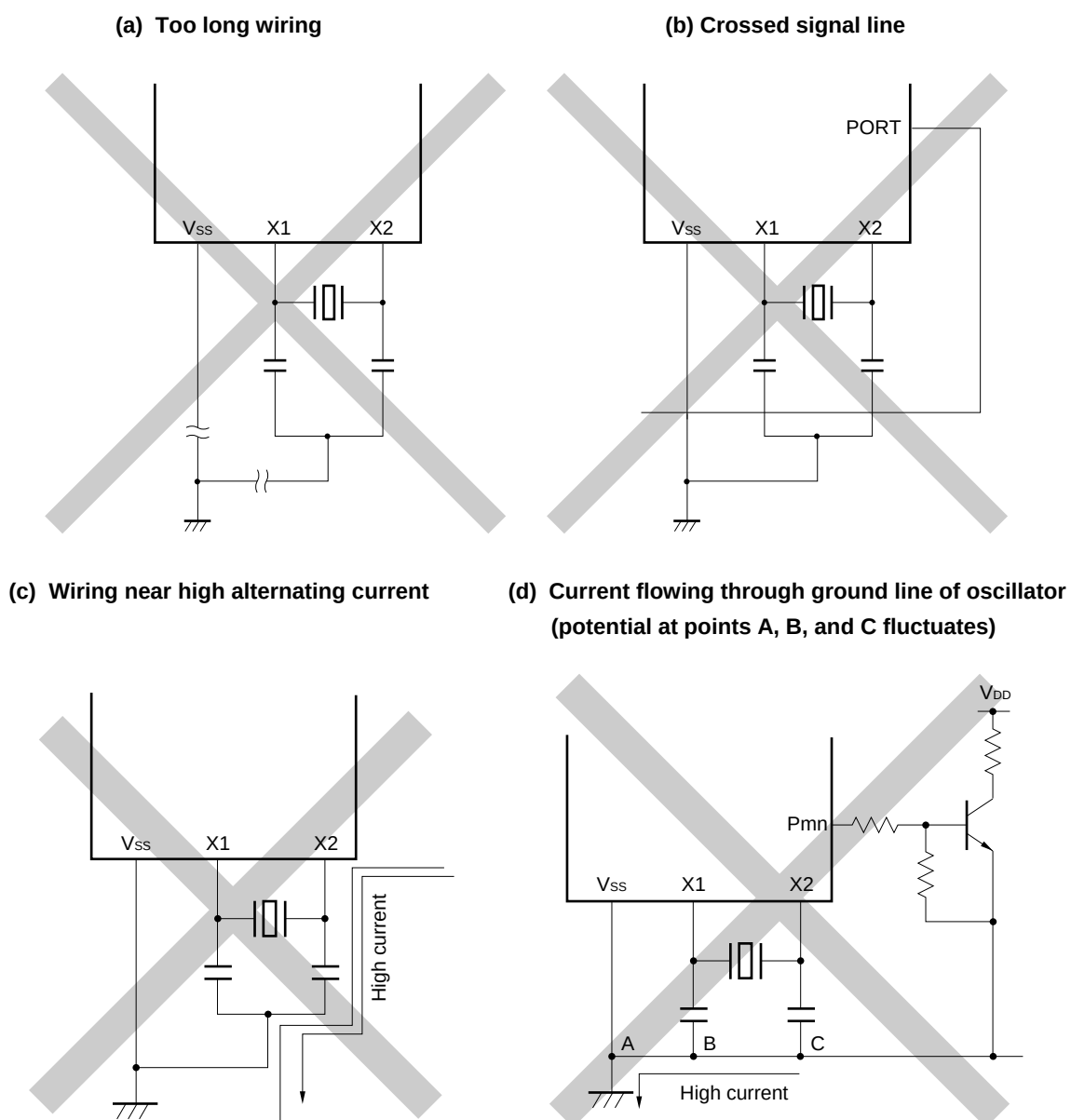
Figure 5-17. Examples of Incorrect Resonator Connection (1/2)
