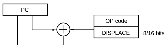
Figure 3-24. Outline of Relative Addressing
