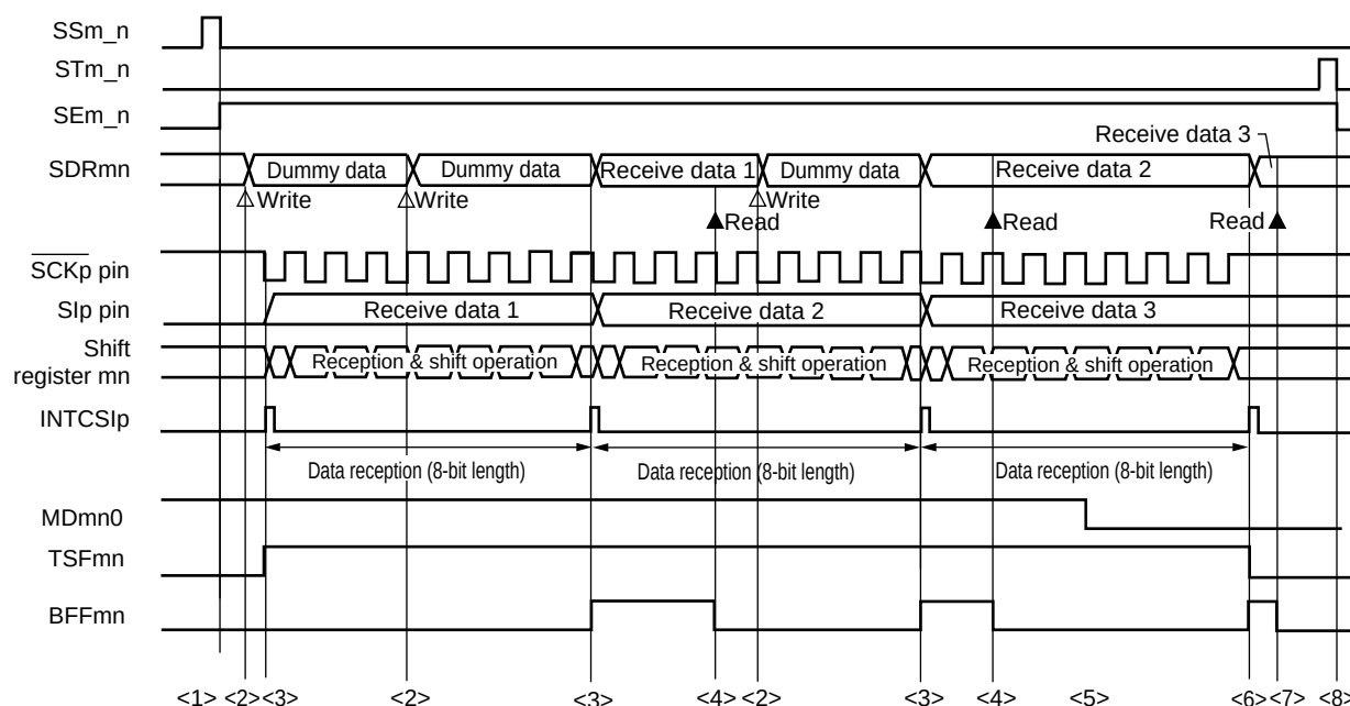
Figure 11-41. Timing Chart of Master Reception (in Continuous Reception Mode)
