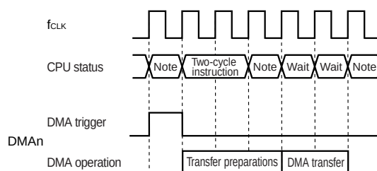
Figure 15-7. Operation Description
