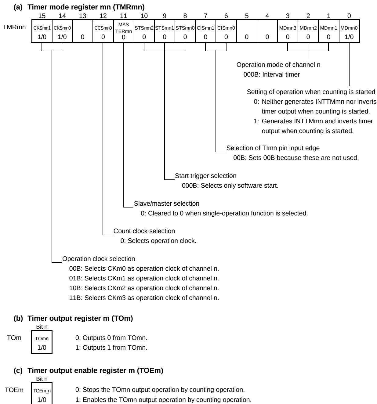
Figure 6-46. Example of Set Contents of Registers During Operation as Interval Timer/Square Wave Output (1/2)
