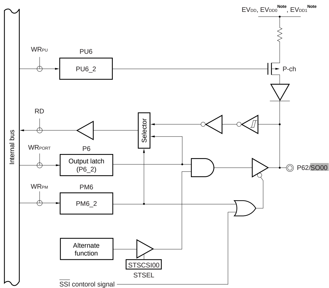
Figure 4-52. Block Diagram of P62
