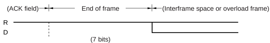
Figure 13-12. End of Frame (EOF)
