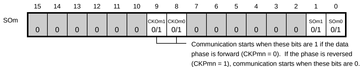
Figure 11-76. Example of Contents of Registers for Master Transmission of SPI Function (CSI00, CSI01) (1/2)
