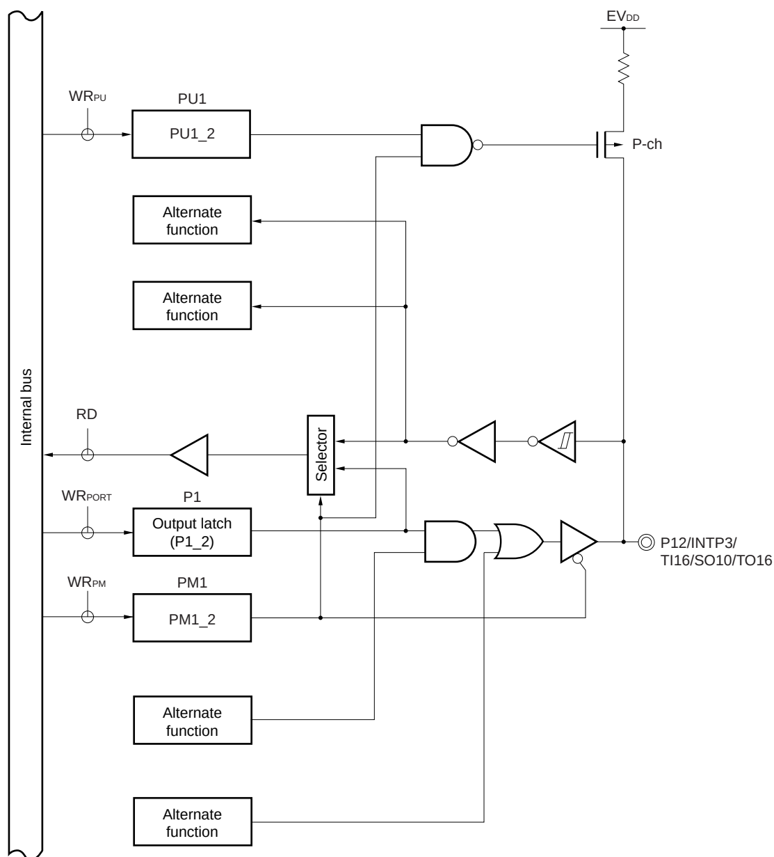
Figure 4-10. Block Diagram of P12 (78K0R/FB3, 78K0R/FC3)
