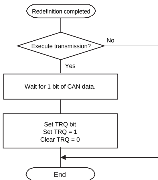
Figure 13-53. Setting Transmission Request (TRQ) to Transmit Message Buffer After Redefining
