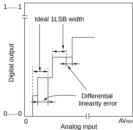
Figure 10-34. Differential Linearity Error
