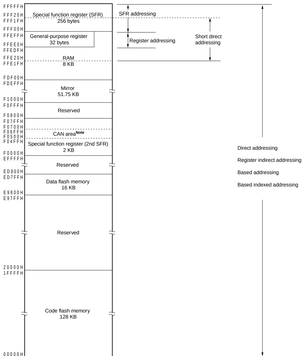
Figure 3-15. Correspondence Between Data Memory and Addressing ( \mu PD78F1817, 78F1822, 78F1825, 78F1828, 78F1833, 78F1838, 78F1843)
