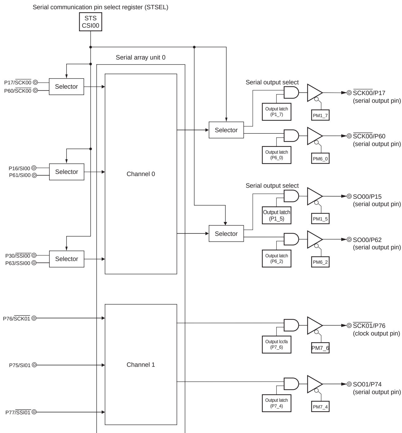
Figure 11-2. Port Configuration Diagram of Serial Array Unit 0
