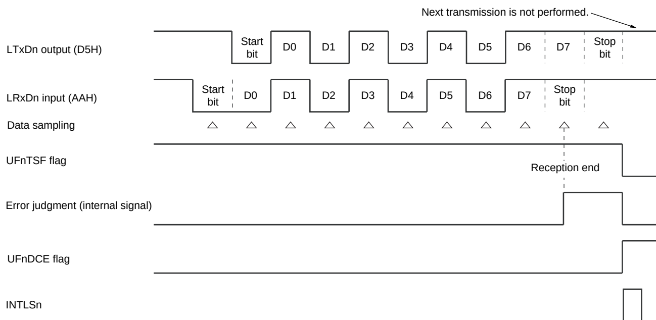
Figure 12-41. Timing Example of Consistency Error Occurrence due to Early End of Reception Processing
