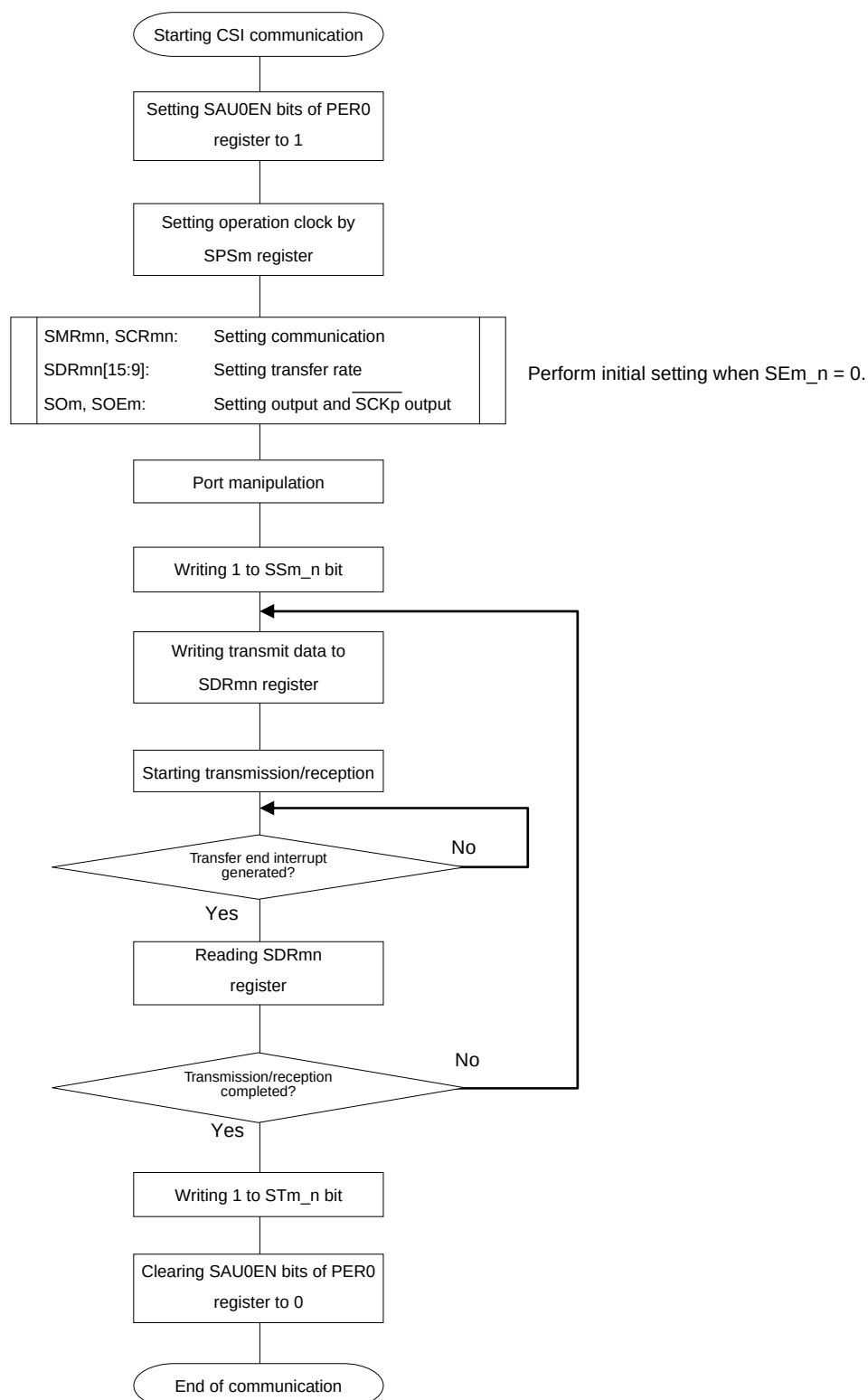
Figure 11-97. Flowchart of Master Transmission/Reception (in Single- Transmission/Reception Mode)
