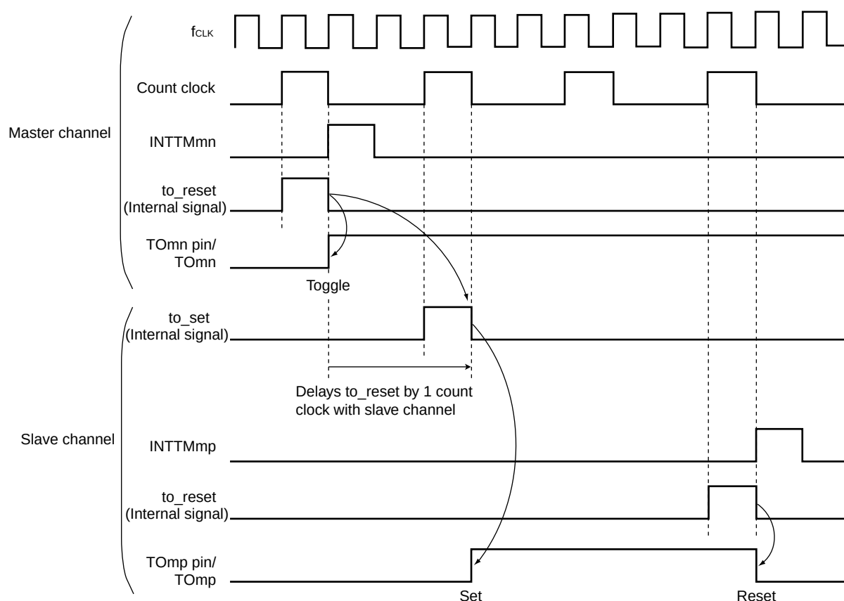
Figure 6-38. Set/Reset Timing Operating Statuses
