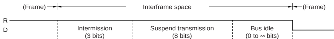
Figure 13-14. Interframe Space (Error Passive Node)
