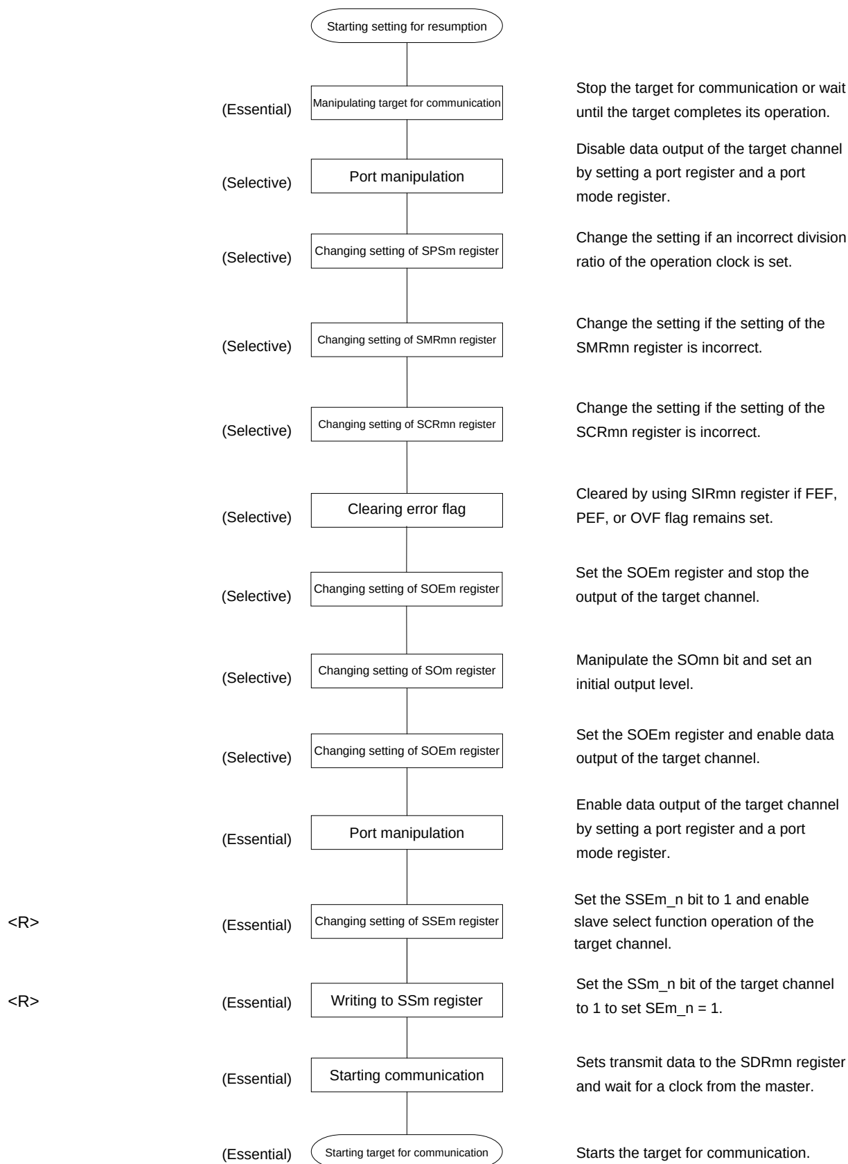
Figure 11-103. Procedure for Resuming Slave Transmission
