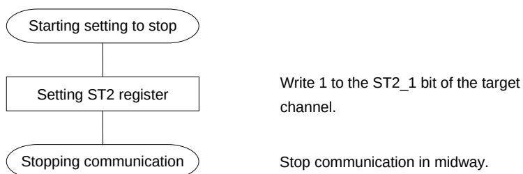
Figure 11-133. Procedure for Stopping UART Reception
