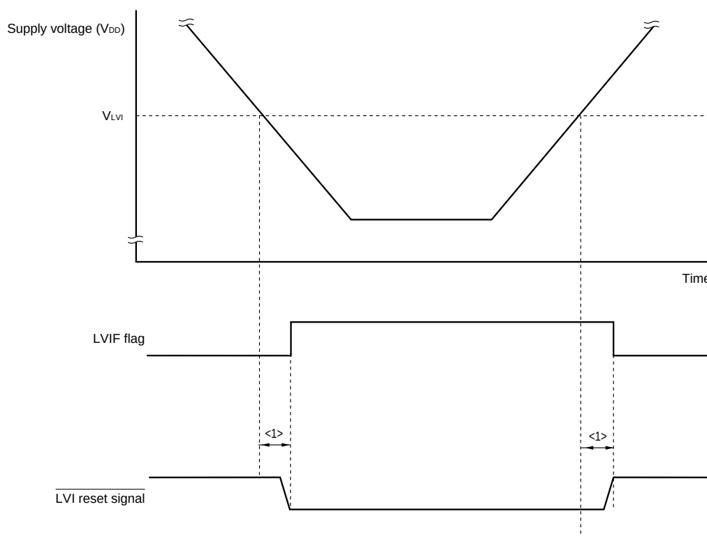
Figure 21-15. Delay from the time LVI reset source is generated until the time LVI reset has been generated or released
