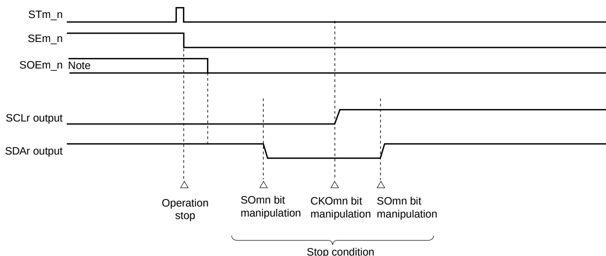
Figure 11-150. Timing Chart of Stop Condition Generation
