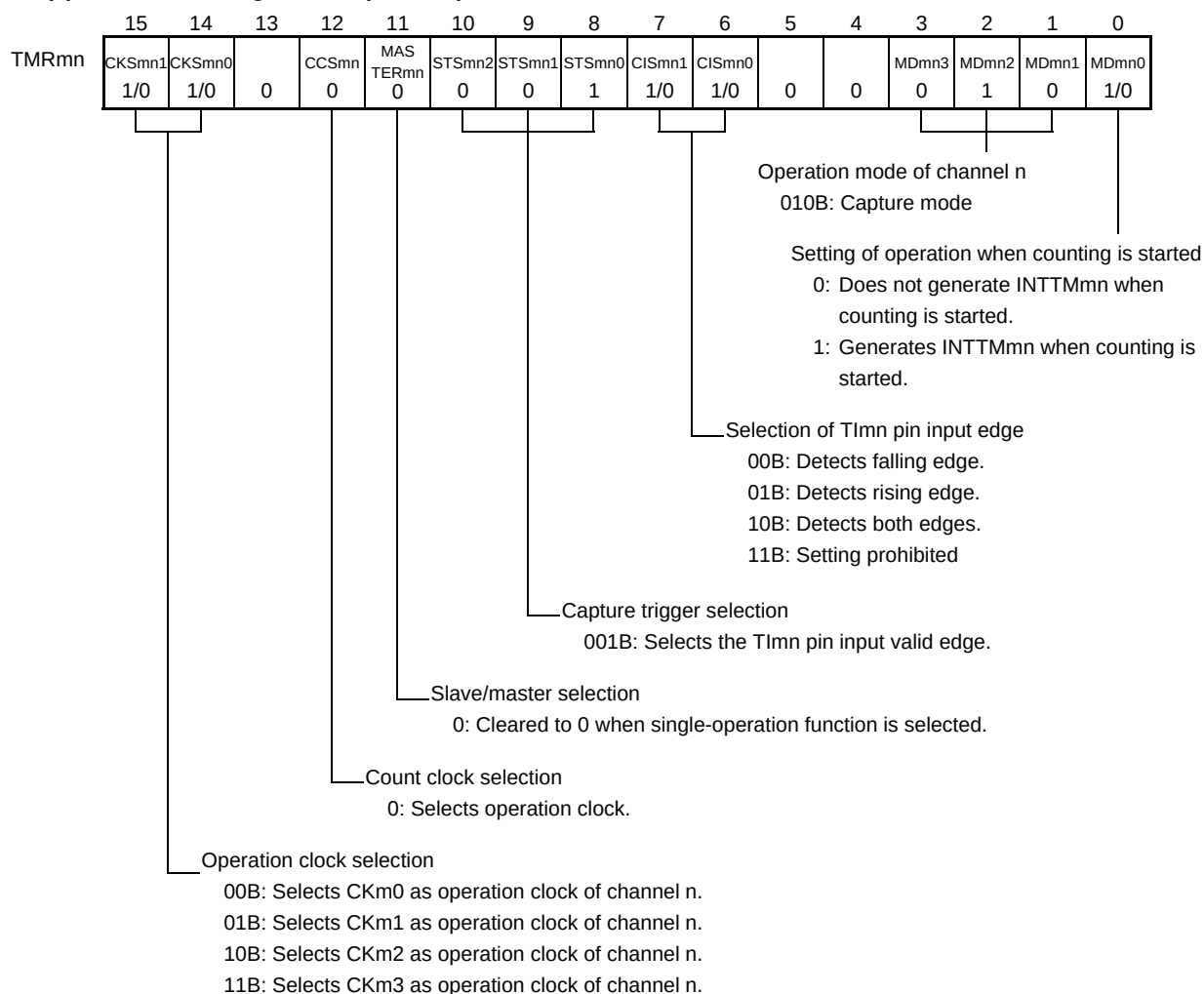
Figure 6-58. Example of Set Contents of Registers to Measure Input Pulse Interval (1/2)
