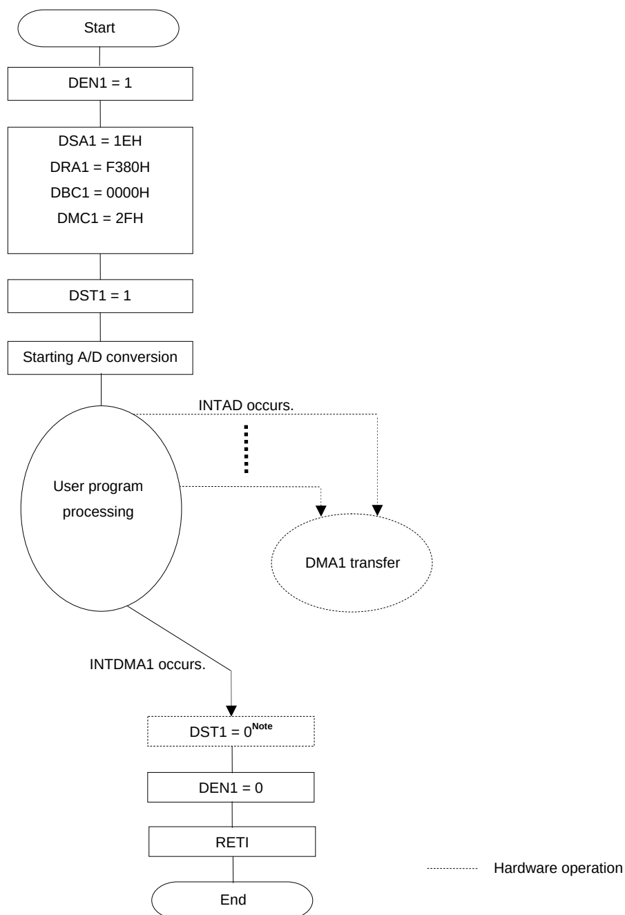
Figure 15-9. Example of Setting of Consecutively Capturing A/D Conversion Results
