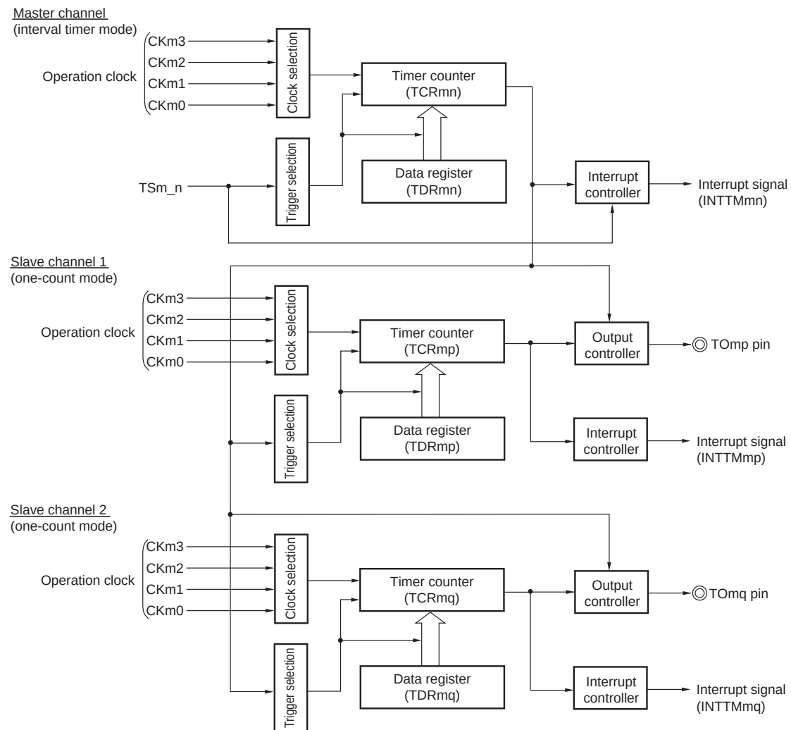
Figure 6-74. Block Diagram of Operation as Multiple PWM Output Function (Output Two Types of PWMs)
