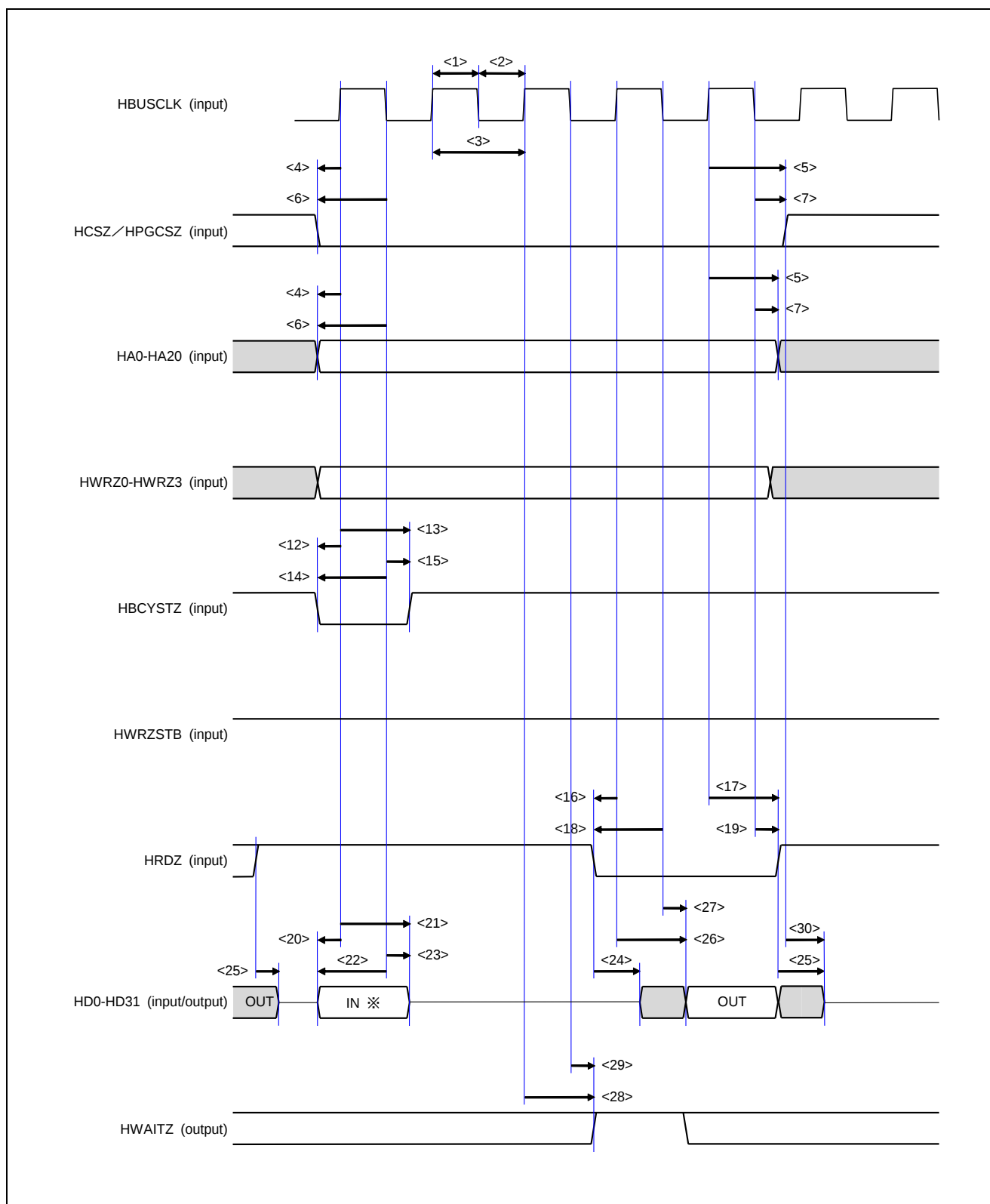
Figure 4.17 External MCU Read Timing (MEMSEL = H, ADMUXMODE = H)
