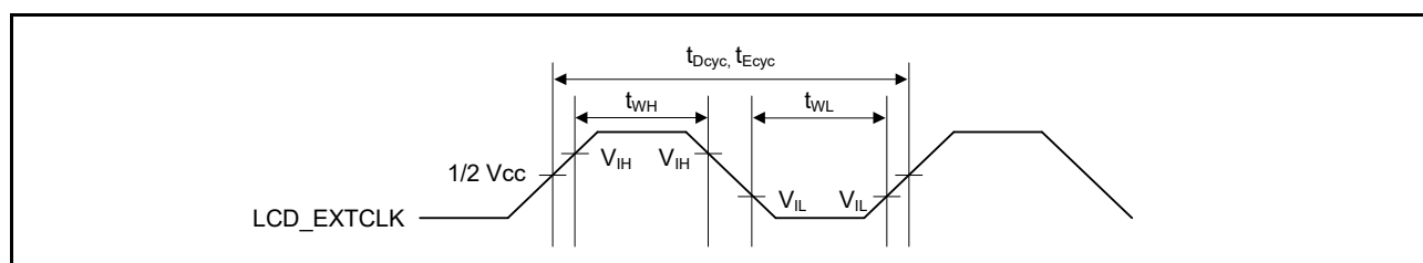
Figure 2.73 LCD_EXTCLK clock input timing
