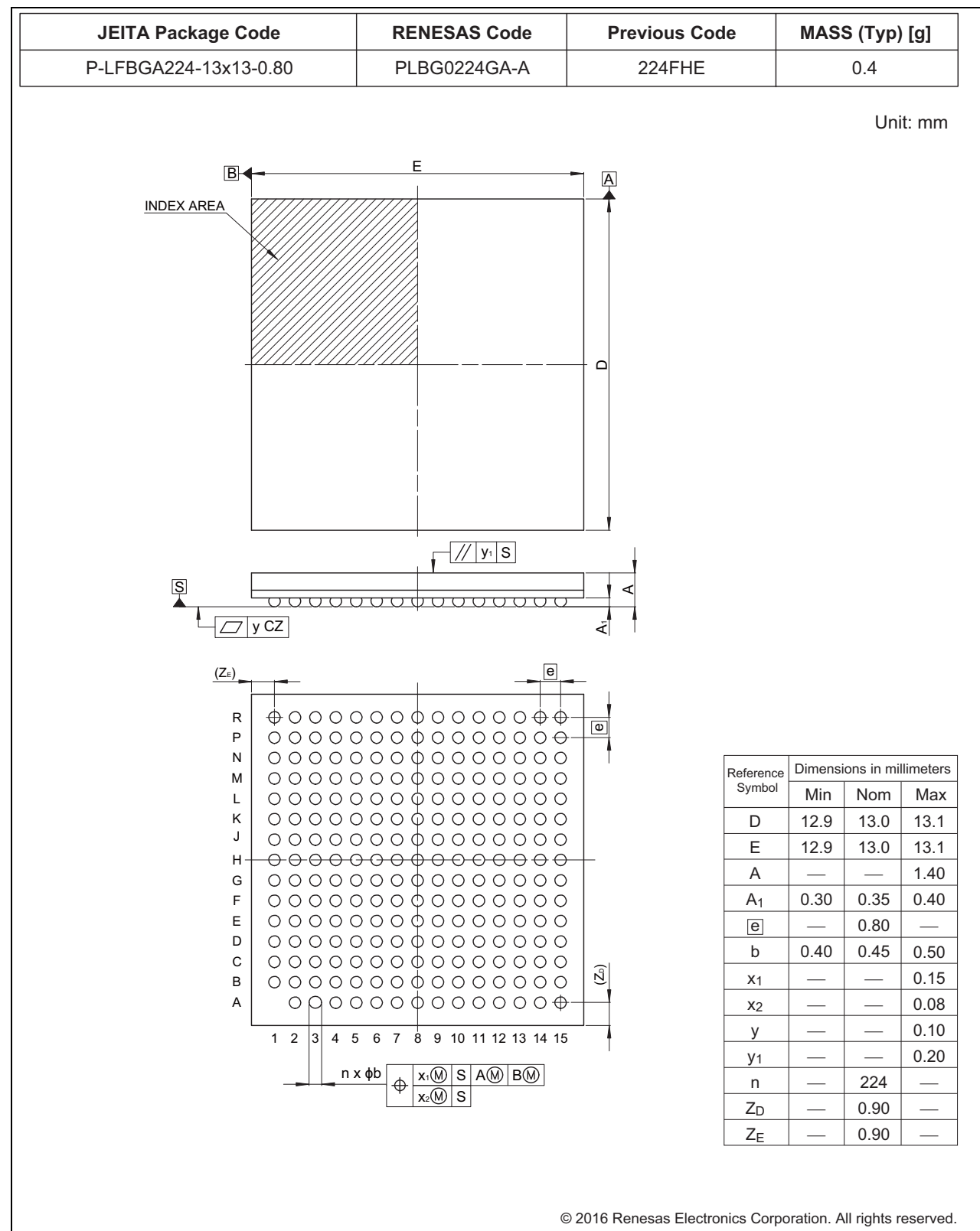
Figure 1.1 224-pin BGA
