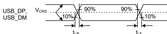
Figure 2.84 USB_DP and USB_DM output timing in low-speed mode
