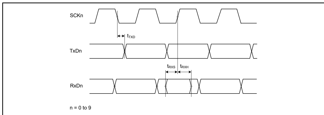
Figure 2.38 SCI input/output timing in clock synchronous mode
