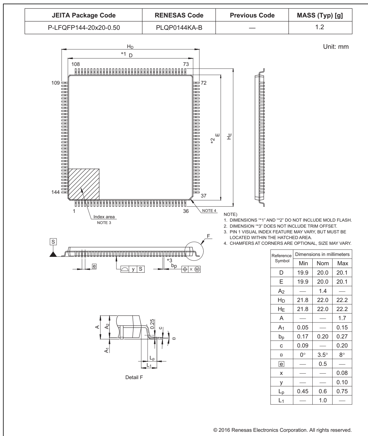
Figure 1.5 144-pin LQFP
