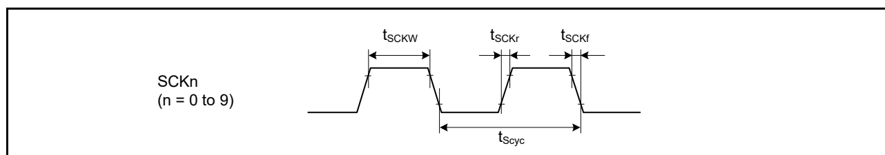
Figure 2.37 SCK clock input/output timing
