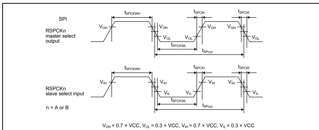
Figure 2.45 SPI clock timing
