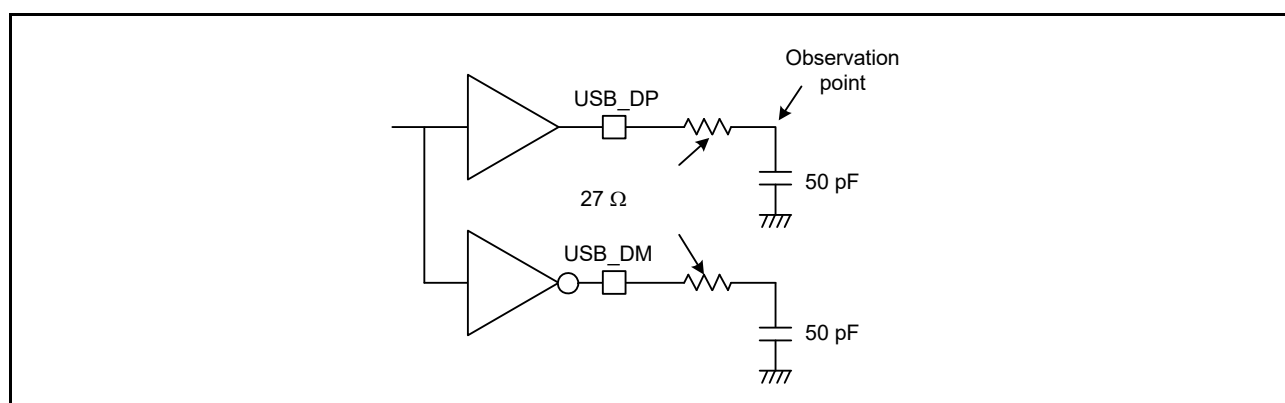
Figure 2.87 Test circuit in full-speed mode
