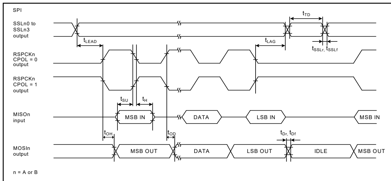
Figure 2.48 SPI timing for master when CPHA = 1
