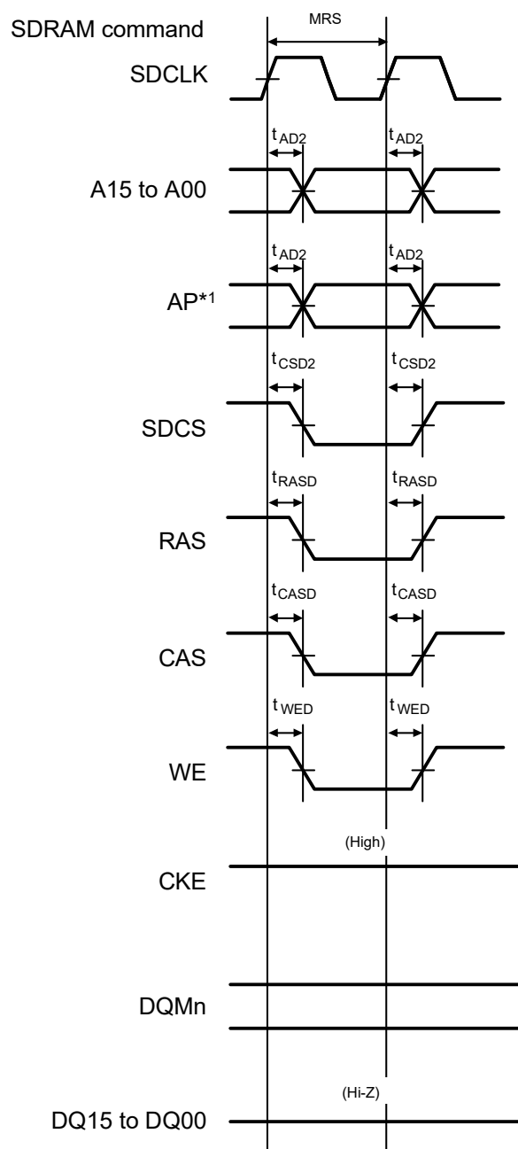
Figure 2.26 SDRAM mode register set timing
