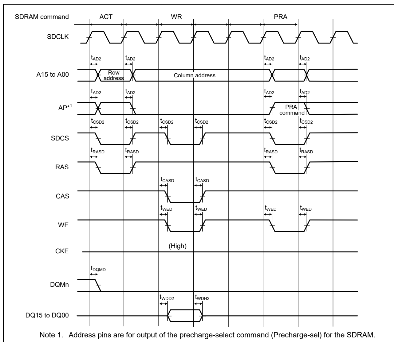
Figure 2.22 SDRAM single write timing
