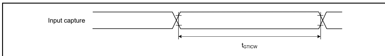
Figure 2.30 GPT32 input capture timing
