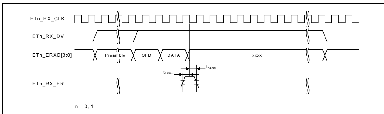
Figure 2.68 MII reception timing when an error occurs
