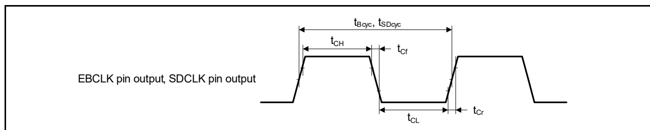
Figure 2.3 EBCLK and SDCLK output timing
