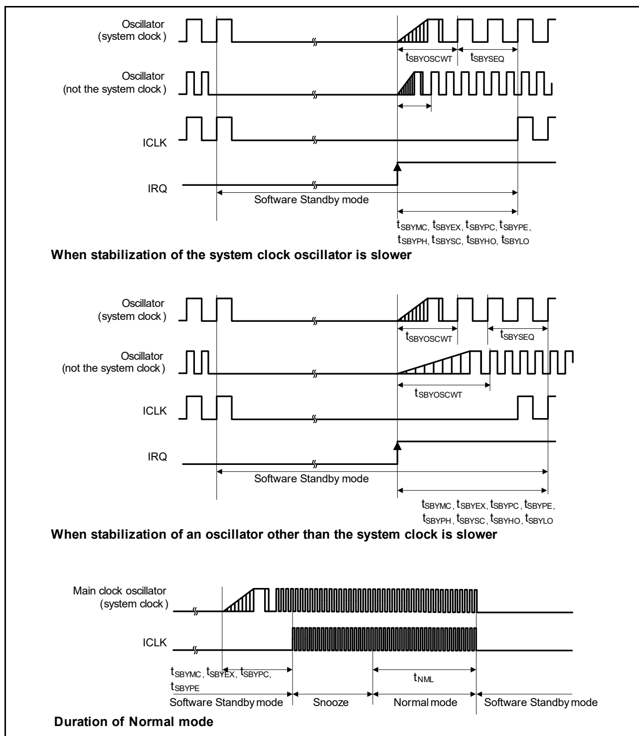
Figure 2.11 Software Standby mode cancellation timing and duration
