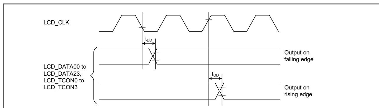
Figure 2.75 Display output timing
