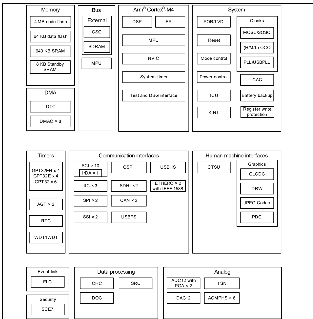
Figure 1.1 Block diagram
