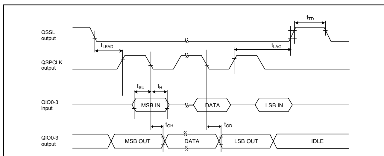
Figure 2.53 Transmit and receive timing
