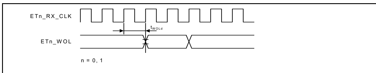
Figure 2.69 WOL output timing for MII
