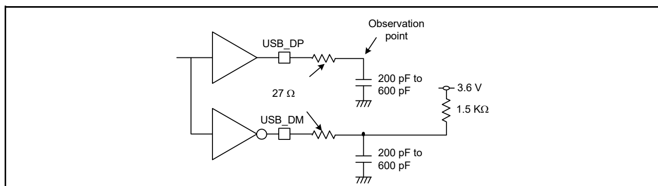
Figure 2.85 Test circuit in low-speed mode
