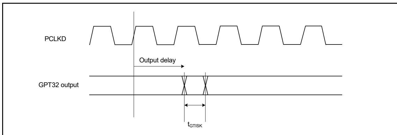
Figure 2.31 GPT32 output delay skew
