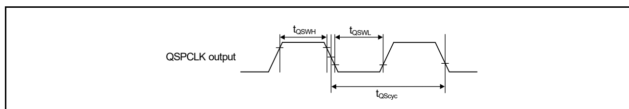
Figure 2.52 QSPI clock timing
