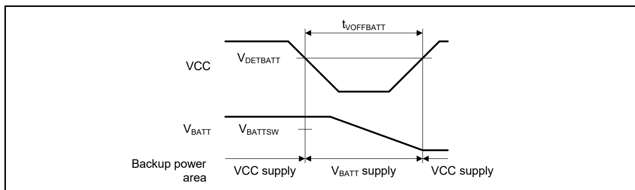
Figure 2.94 Battery backup function characteristics
