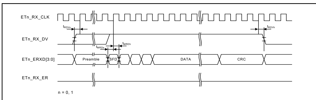
Figure 2.67 MII reception timing in normal operation
