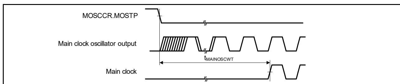
Figure 2.5 Main clock oscillation start timing
