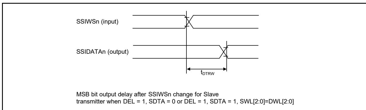
Figure 2.58 SSI data output delay after SSIWSn change
