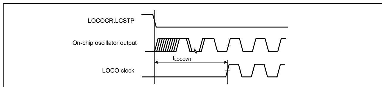
Figure 2.6 LOCO clock oscillation start timing
