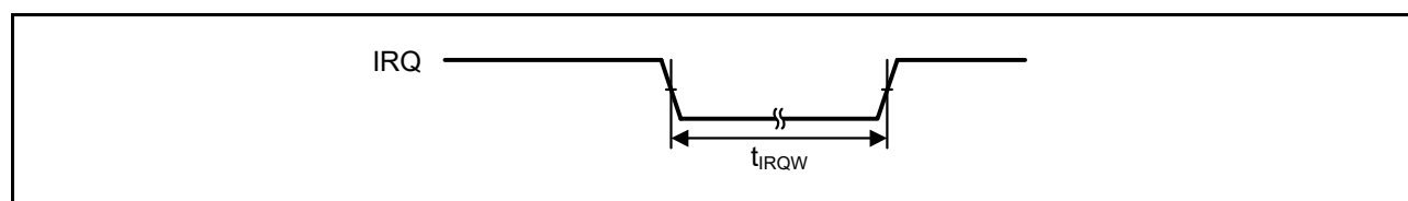
Figure 2.15 IRQ interrupt input timing
