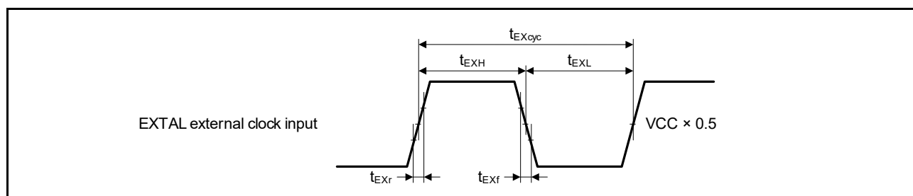
Figure 2.4 EXTAL external clock input timing
