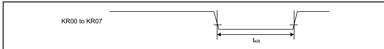
Figure 2.36 Key interrupt input timing
