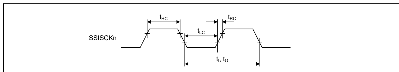
Figure 2.55 SSI clock input/output timing
