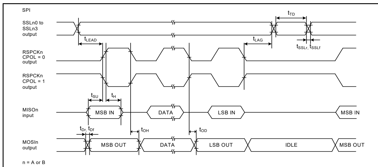
Figure 2.46 SPI timing for master when CPHA = 0
