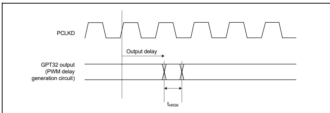
Figure 2.33 GPT32 (PWM Delay Generation Circuit) output delay skew
