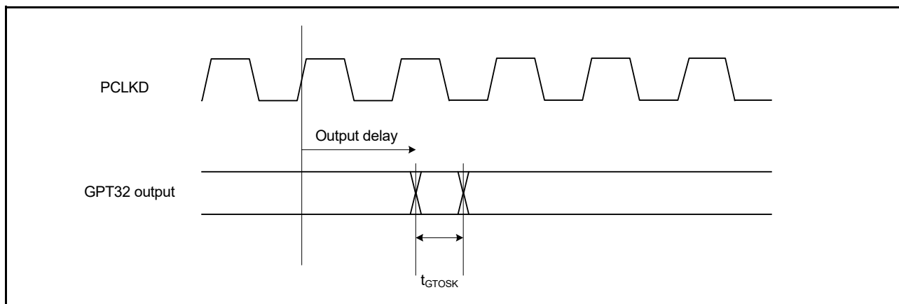
Figure 2.32 GPT32 output delay skew for OPS
