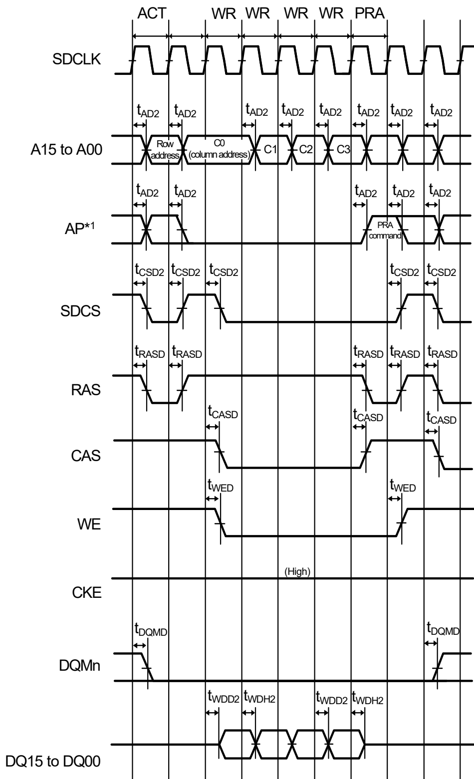
Figure 2.24 SDRAM multiple write timing
