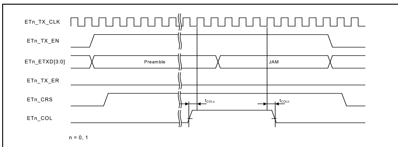
Figure 2.66 MII transmission timing when a conflict occurs
