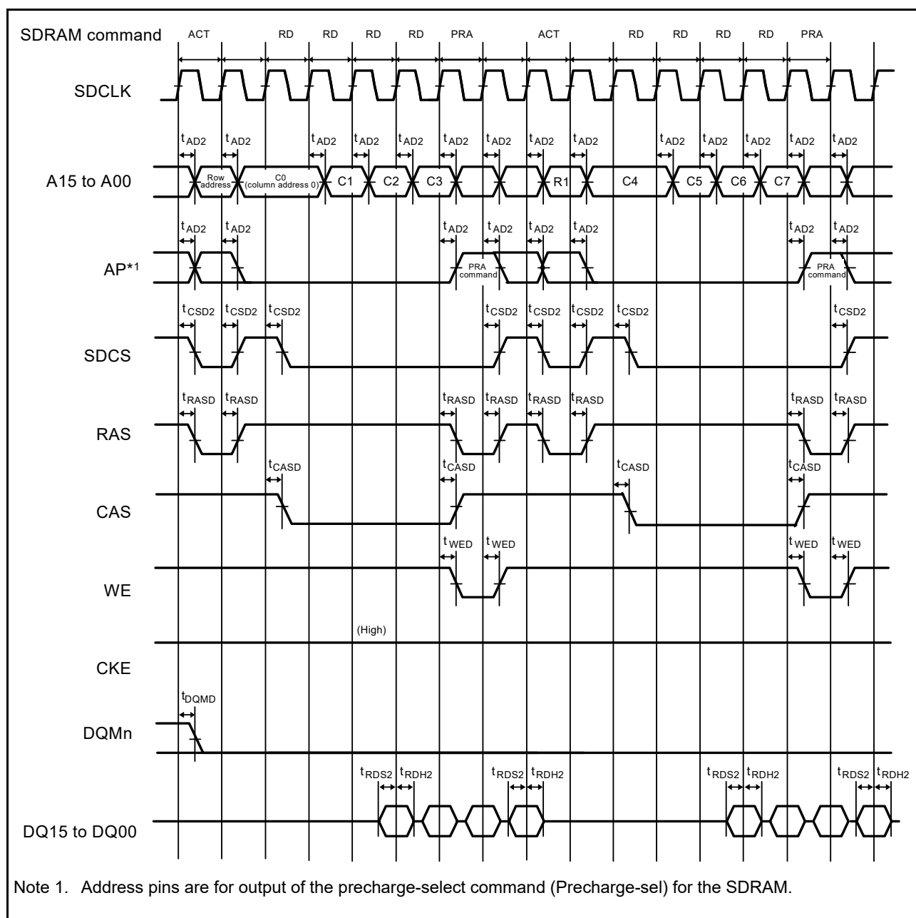
Figure 2.25 SDRAM multiple read line stride timing
