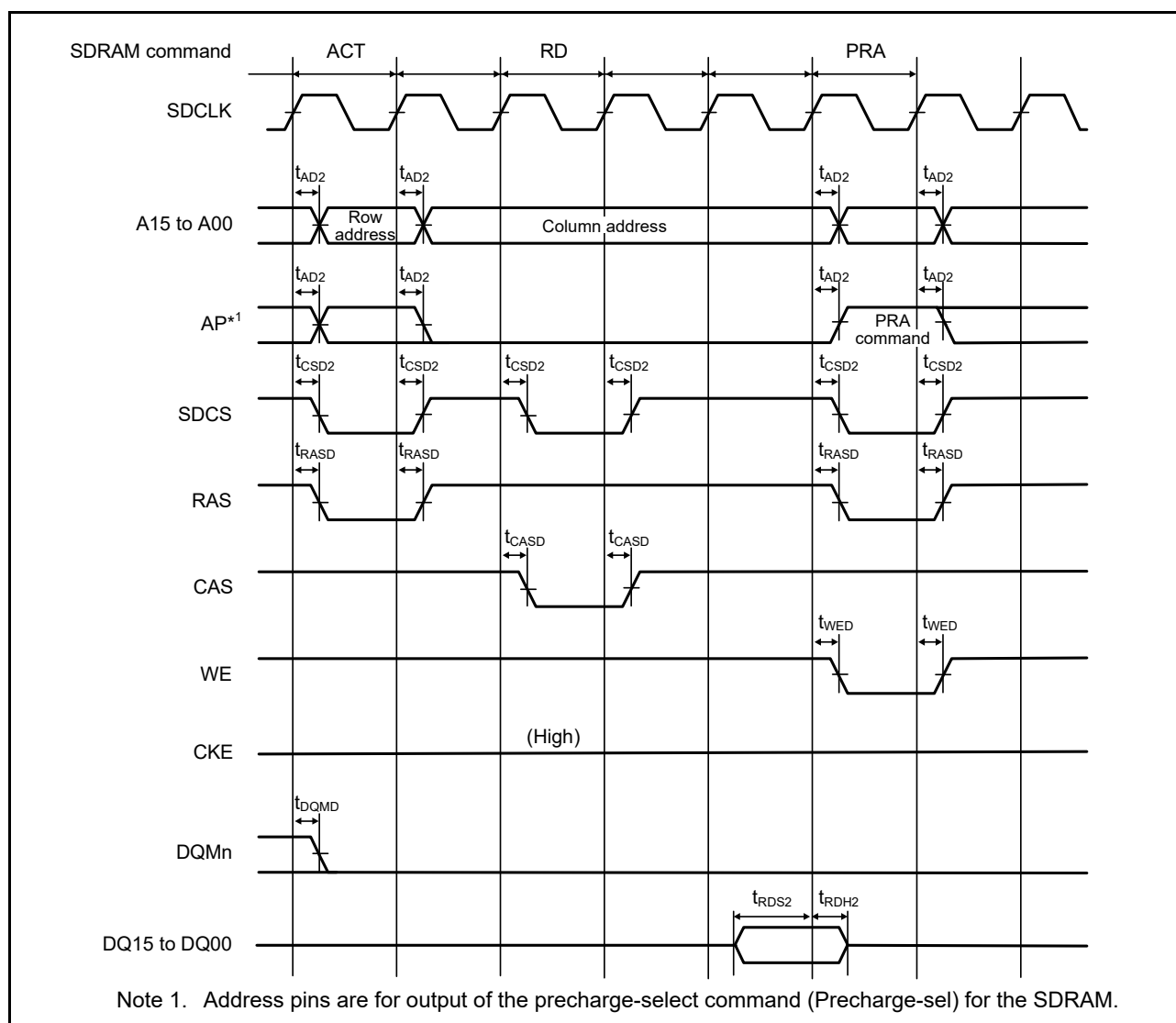
Figure 2.21 SDRAM single read timing
