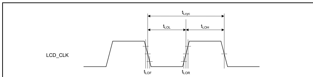
Figure 2.74 LCD_CLK clock output timing
