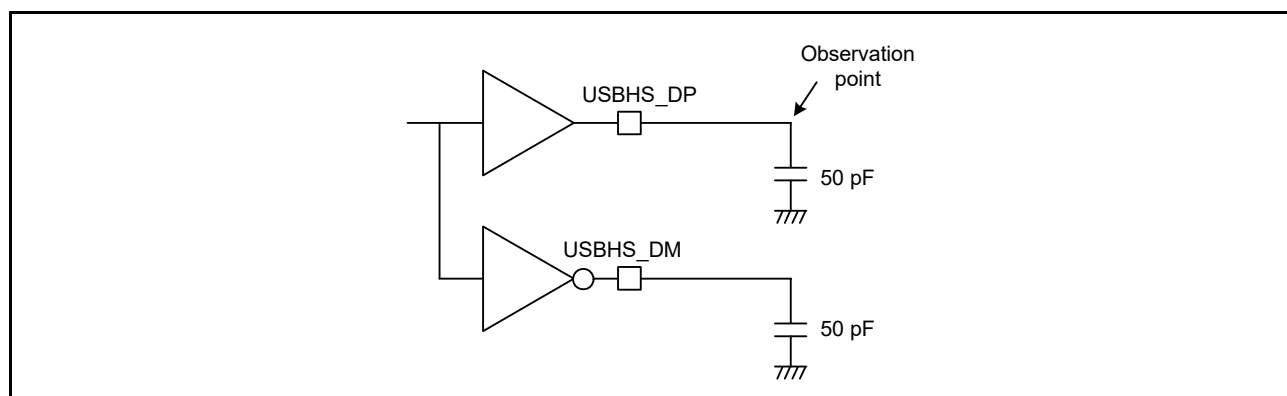
Figure 2.79 Test circuit in full-speed mode
