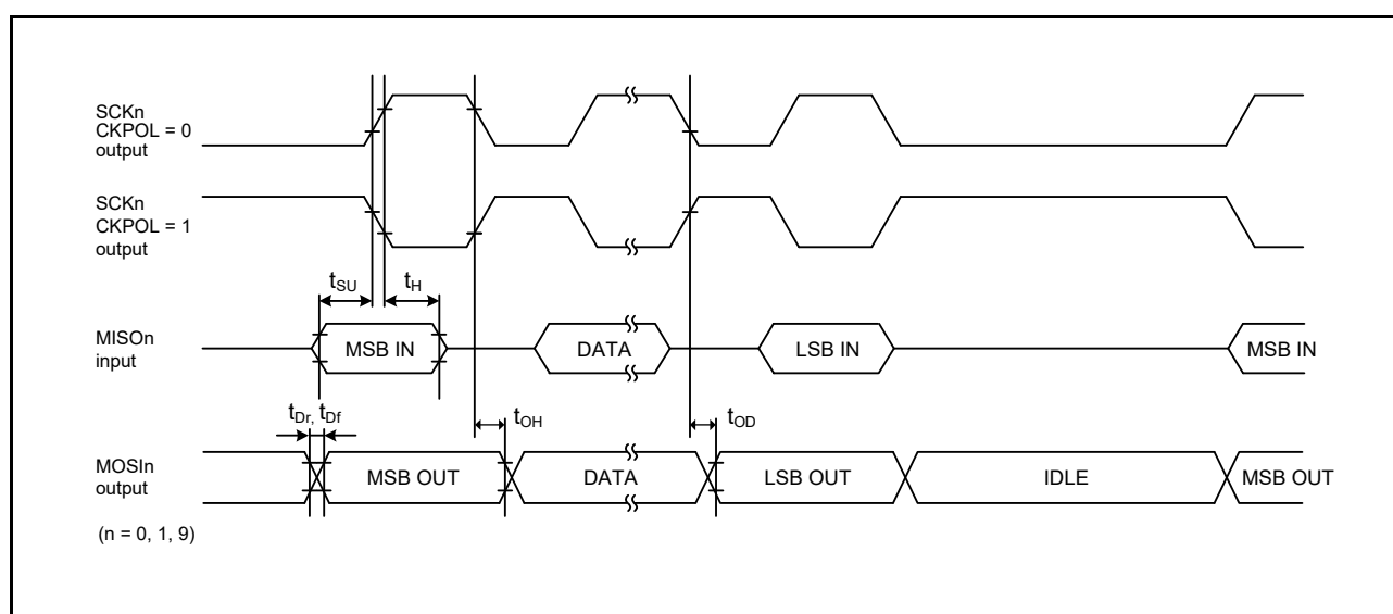
Figure 2.44 SCl simple SPI mode timing (master, CKPH = 1)
