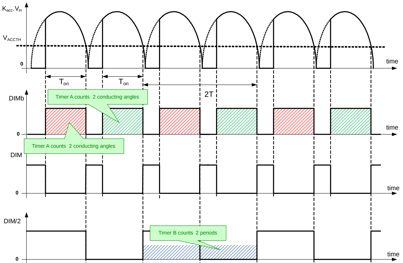
Figure 35. Time diagram of the implemented conduction angle measurement
