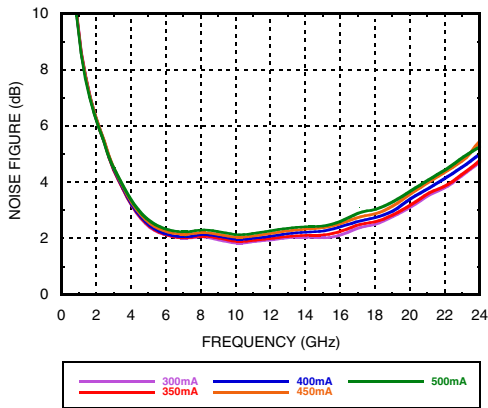
Noise Figure vs. Idq
