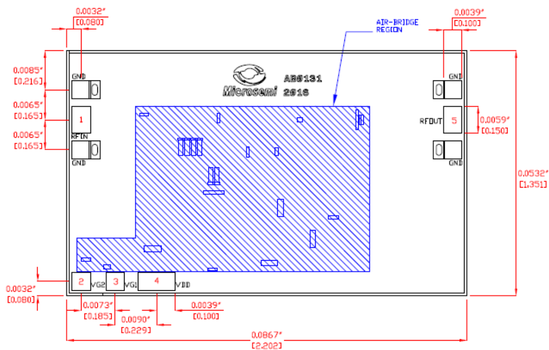
Figure 14 Chip Outline
