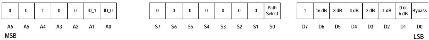
Figure 105. I3C Word
