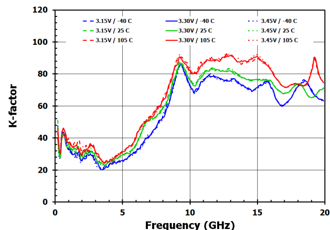
Figure 18. Stability K-factor
