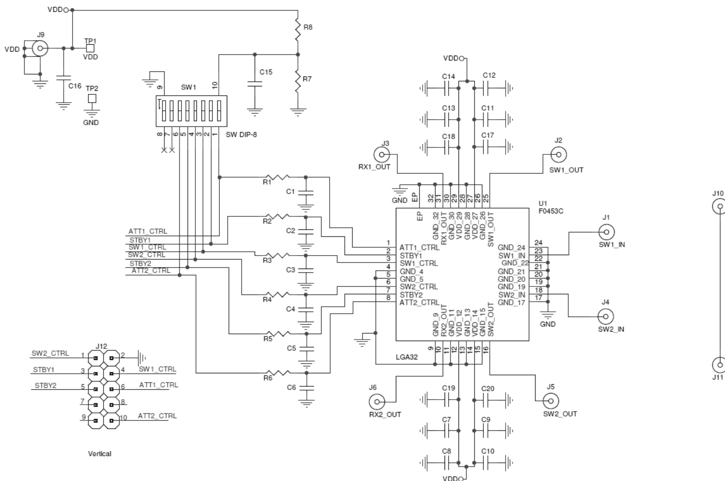
Figure 27. Electrical Schematic
