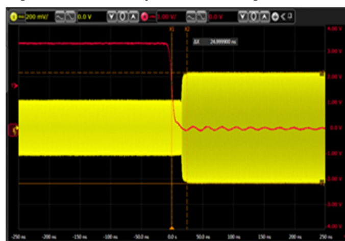
Figure 20. Gain Step Phase Settling Time
