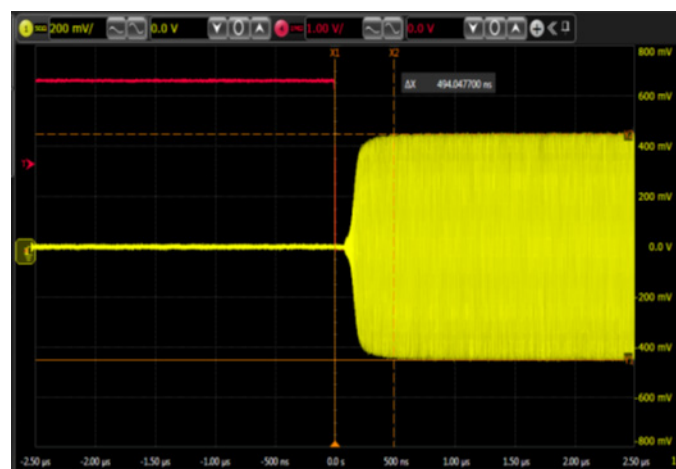
Figure 24. Power ON from Standby Mode
