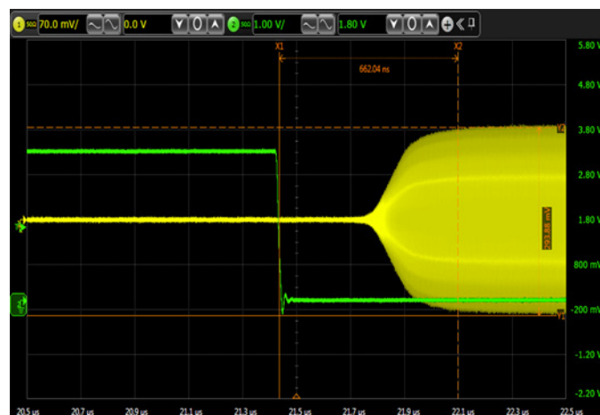
Figure 22. Power ON Switching Time
