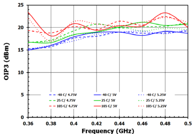
Figure 44. LB Output IP3 for DSA0 = 0dB, DSA1 = 0dB, DSA2 = 18dB, and Pout = -18dBm/tone
