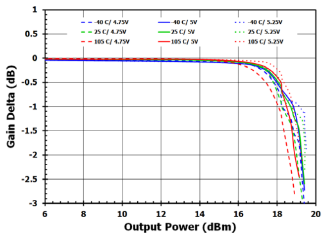
Figure 46. Gain Compression [400MHz]
