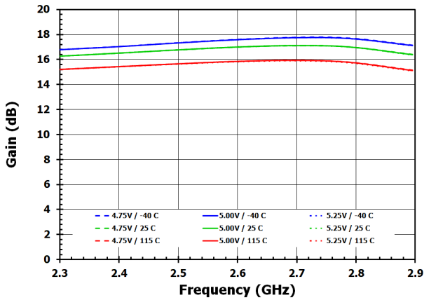
Figure 2. Gain
