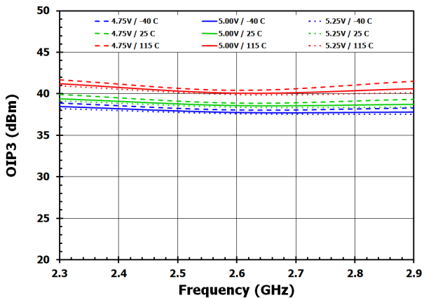
Figure 6. OIP3
