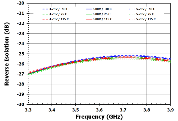
Figure 11. Reverse Isolation
