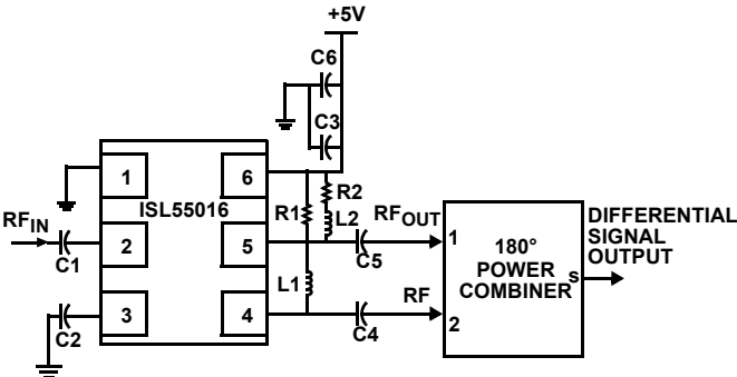
FIGURE 33. EVALUATION BOARD WITH 2-WAY 180° POWER COMBINER
