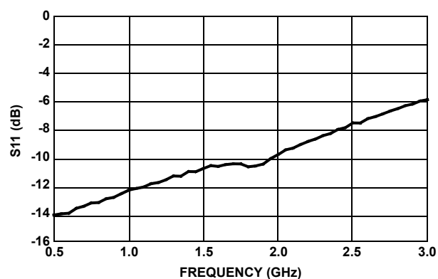
FIGURE 6. |S_{11}| vs FREQUENCY
