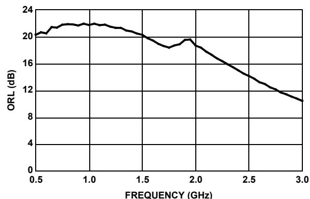
FIGURE 4. OUTPUT RETURN LOSS vs FREQUENCY
