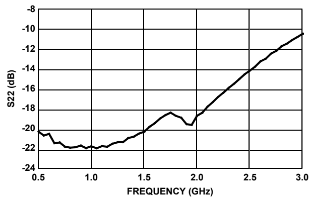
FIGURE 8. |S_{22}| vs FREQUENCY
