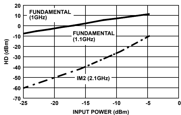
FIGURE 10. IM2 vs INPUT POWER
