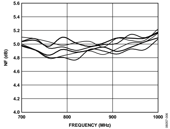
Figure 6. Noise Figure vs. Frequency, Multiple Devices, V_S = 5V , T_A = 25^\circ\text{C}
