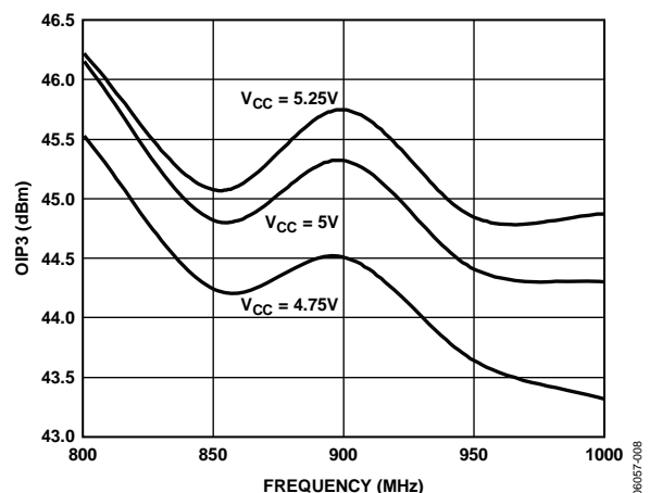
Figure 8. OIP3 vs. Frequency, V_{CC} = 4.75V , 5V , and 5.25V , T_A = 25^\circ\text{C}
