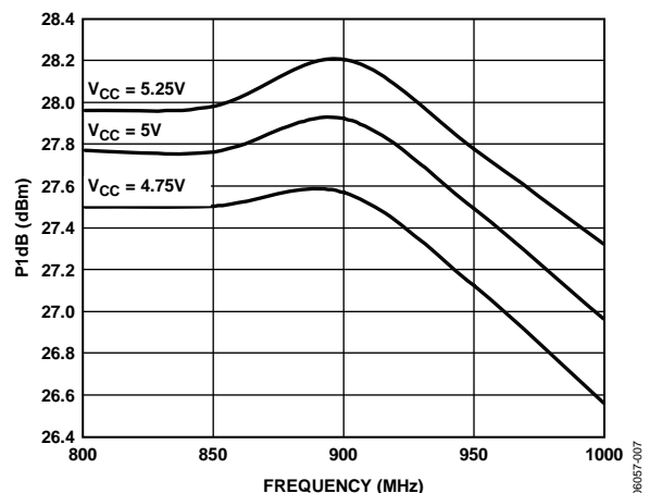
Figure 7. P1 dB vs. Frequency, V_{CC} = 4.75V , 5V , and 5.25V , T_A = 25^\circ\text{C}
