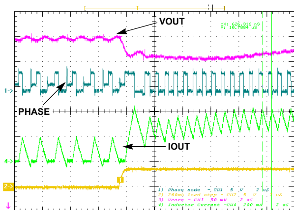
50mA to 260mA load step on V_{\text{OUT}} . Top: Output voltage, 50mV/DIV; Phase node, 5V/DIV; Inductor current, 200mA/DIV, 2 \mu\text{s} /DIV
