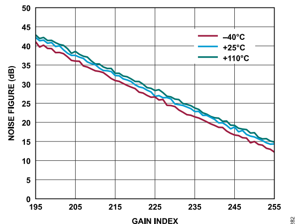
Figure 153. Receiver Noise Figure vs. Gain Index, Baseband Frequency = 5.6 MHz, ADC = Low Power
