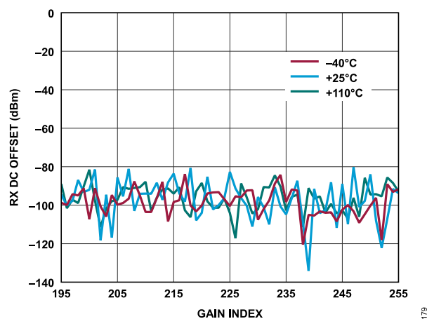
Figure 75. Receiver DC Offset vs. Gain Index, Baseband Frequency = 5.6 MHz, ADC = High Performance
