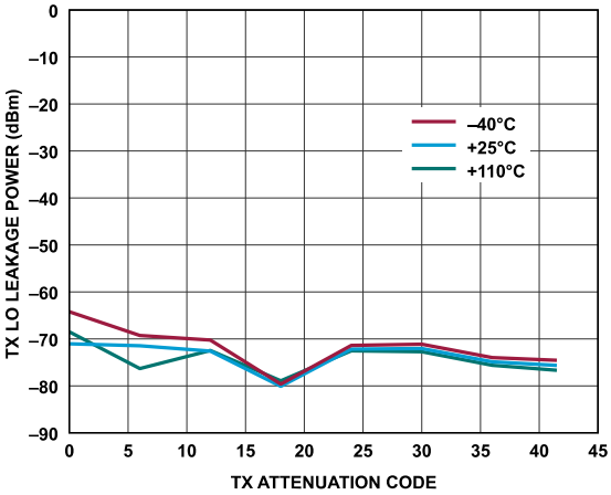
Figure 271. Transmitter LO Leakage Power vs. Transmitter Attenuation Code, Baseband Frequency = 2.1 kHz, Backoff = 6 dBFS, Initialization Calibration Only
