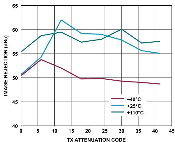
Figure 144. Transmitter Image Rejection vs. Transmitter Attenuation Code, Baseband Frequency = 18 MHz, Backoff = 0.2 dBFS, Initialization Calibration Only
