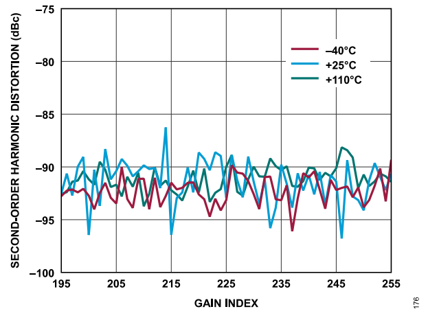
Figure 69. Receiver Second-Order Harmonic Distortion vs. Gain Index, Baseband Frequency = 5.6 MHz, ADC = Low Power
