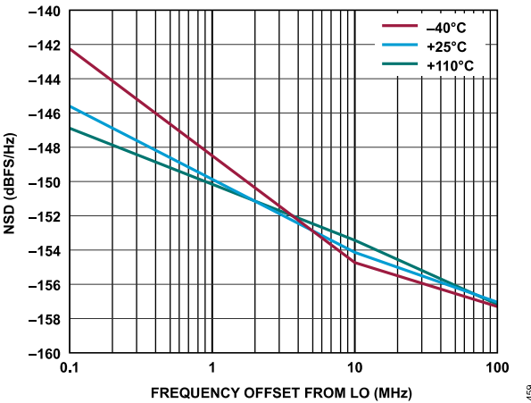
Figure 253. Transmitter NSD vs. Frequency Offset from LO, Baseband Frequency = 2.1 kHz, Transmitter Channel = Ch1
