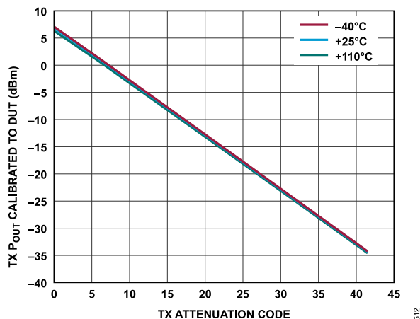
Figure 285. Transmitter Absolute Power vs. Transmitter Attenuation Code, Baseband Frequency = 2.1 kHz, Backoff = 0.2 dBFS
