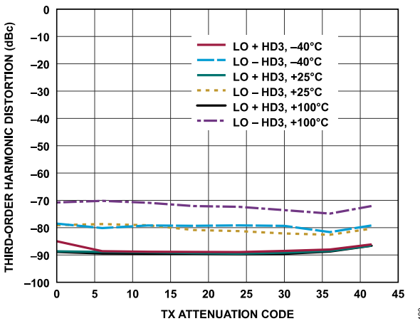
Figure 269. Transmitter Third-Order Harmonic Distortion vs. Transmitter Attenuation Code, Baseband Frequency = 2.1 kHz, Backoff = 0.2 dBFS
