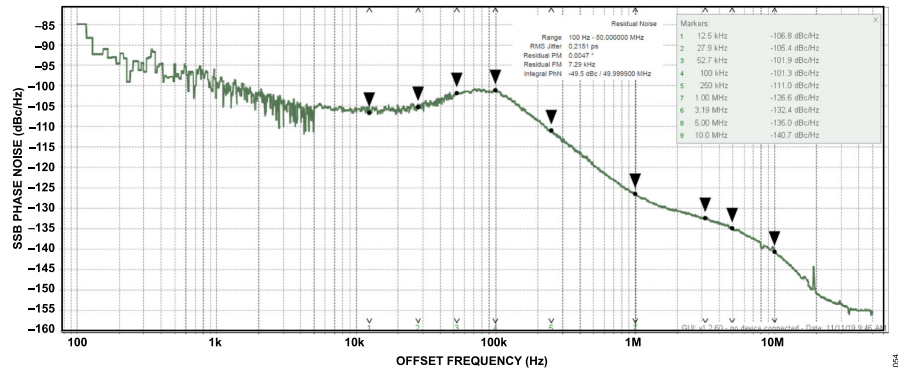
Figure 296. Internal Local Oscillator Phase Noise at 3500 MHz LO
