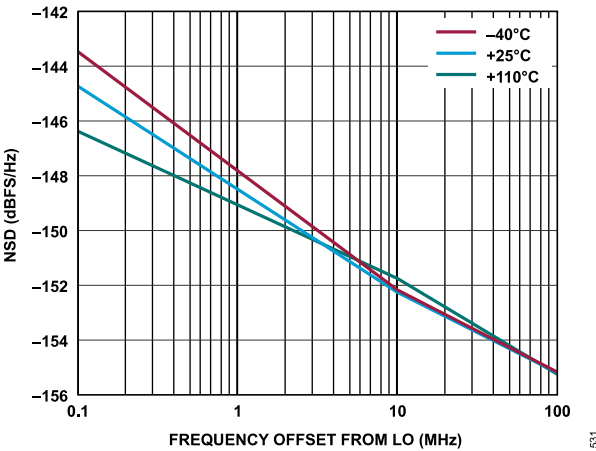
Figure 291. Transmitter NSD vs. Frequency Offset from LO, Baseband Frequency = 2.1 kHz, Transmitter Channel = Ch1
