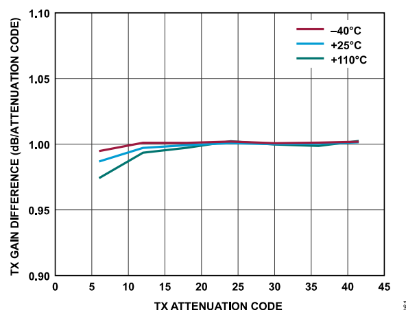
Figure 141. Transmitter Attenuation Delta (Error) vs. Transmitter Attenuation Code, Baseband Frequency = 18 MHz, Backoff = 0.2 dBFS
