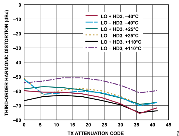
Figure 145. Transmitter Third-Order Harmonic Distortion vs. Transmitter Attenuation Code, Baseband Frequency = 18 MHz, Backoff = 0.2 dBFS
