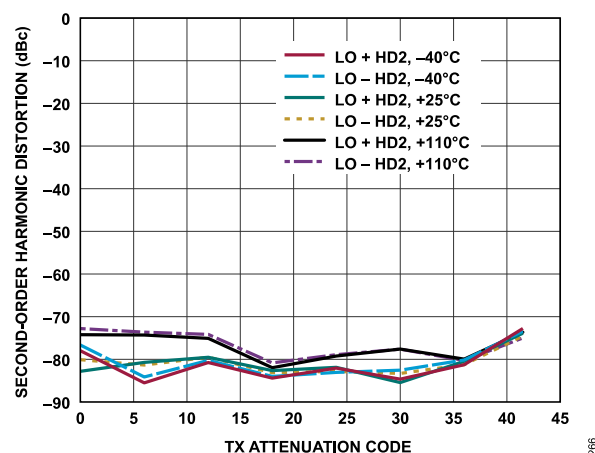
Figure 146. Transmitter Second-Order Harmonic Distortion vs. Transmitter Attenuation Code, Baseband Frequency = 18 MHz, Backoff = 0.2 dBFS
