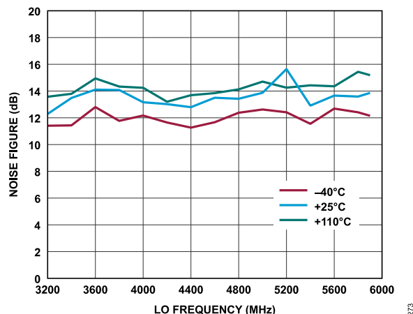
Figure 123. Receiver Noise Figure vs. LO Frequency, Baseband Frequency = 5.6 MHz, ADC = Low Power
