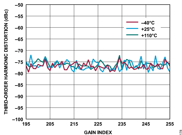
Figure 73. Receiver Third-Order Harmonic Distortion vs. Gain Index, Baseband Frequency = 5.6 MHz, ADC = Low Power
