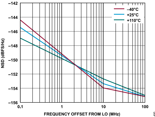
Figure 272. Transmitter NSD vs. Frequency Offset from LO, Baseband Frequency = 2.1 kHz, Transmitter Channel = Ch1
