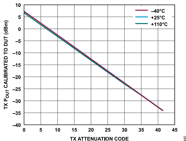
Figure 247. Transmitter Absolute Power vs. Transmitter Attenuation Code, Baseband Frequency = 2.1 kHz, Backoff = 0.2 dBFS
