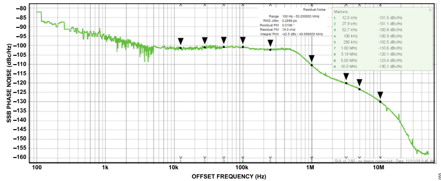
Figure 297. Internal Local Oscillator Phase Noise at 5800 MHz LO
