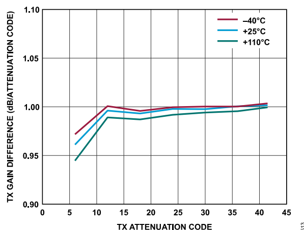
Figure 286. Transmitter Attenuation Delta (Error) vs. Transmitter Attenuation Code, Baseband Frequency = 2.1 kHz, Backoff = 0.2 dBFS
