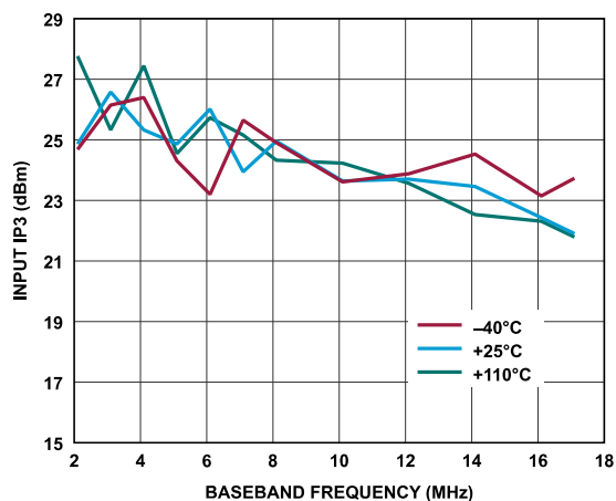
Figure 77. Receiver Input IP3 vs. Baseband Frequency, ADC = Low Power, F1 = Baseband Frequency, F2 = Baseband Frequency + 1 MHz, Gain Index = 255
