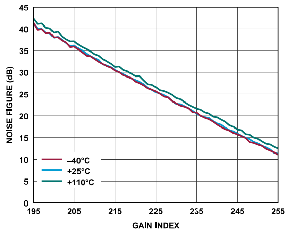
Figure 217. Receiver Noise Figure vs. Gain Index, Baseband Frequency = 2.1 kHz, ADC = High Performance
