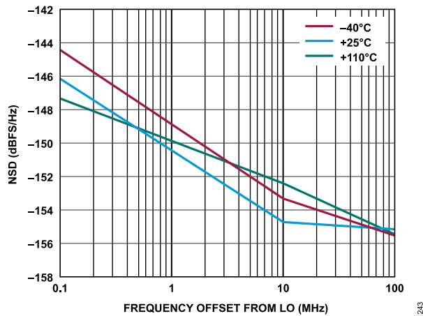
Figure 117. Transmitter NSD vs. Frequency Offset from LO, Baseband Frequency = 5.6 MHz, Transmitter Channel = Ch1
