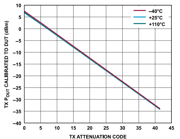
Figure 167. Transmitter Absolute Power vs. Transmitter Attenuation Code, Baseband Frequency = 18 MHz, Backoff = 0.2 dBFS
