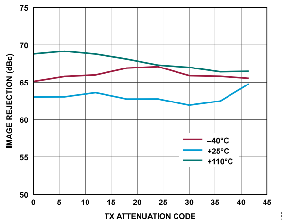
Figure 57. Transmitter Image Rejection vs. Transmitter Attenuation Code, Baseband Frequency = 18 MHz, Backoff = 0.2 dBFS, Initialization Calibration Only
