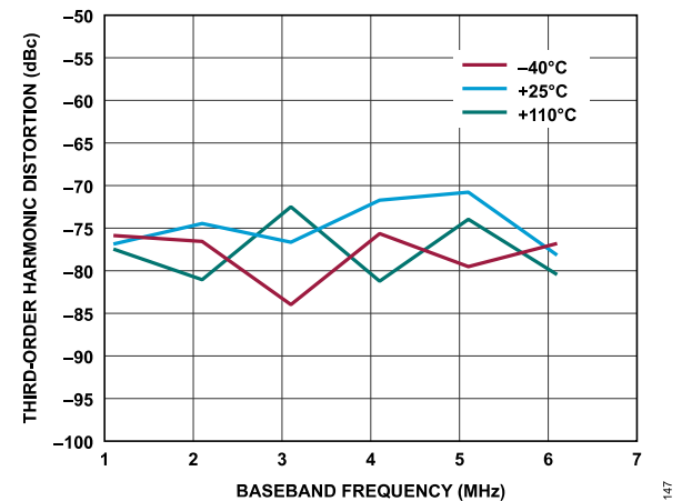
Figure 47. Receiver Third-Order Harmonic Distortion vs. Baseband Frequency, Gain Index = 255, ADC = Low Power
