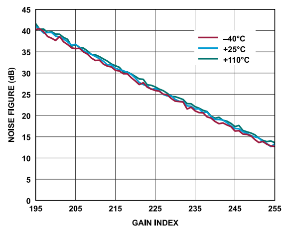
Figure 152. Receiver Noise Figure vs. Gain Index, Baseband Frequency = 5.6 MHz, ADC = High Performance
