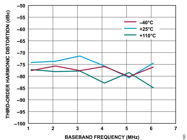
Figure 74. Receiver Third-Order Harmonic Distortion vs. Baseband Frequency, Gain Index = 255, ADC = Low Power
