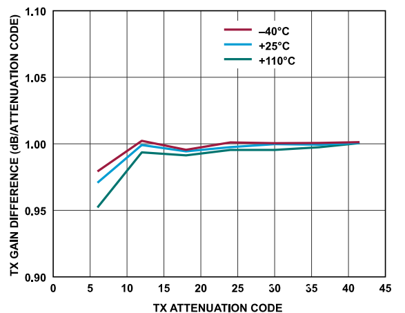
Figure 168. Transmitter Attenuation Delta (Error) vs. Transmitter Attenuation Code, Baseband Frequency = 18 MHz, Backoff = 0.2 dBFS
