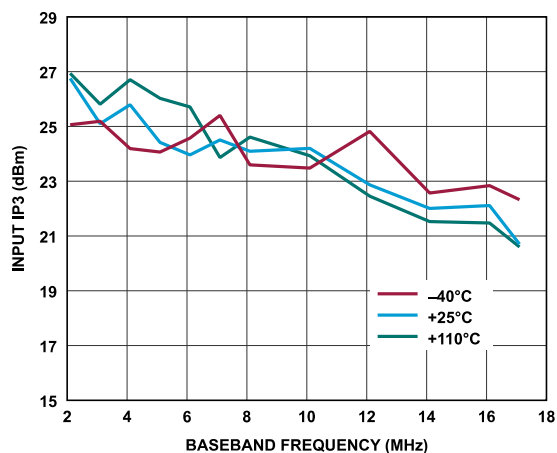
Figure 104. Receiver Input IP3 vs. Baseband Frequency, ADC = Low Power, F1 = Baseband Frequency, F2 = Baseband Frequency + 1 MHz, Gain Index = 255
