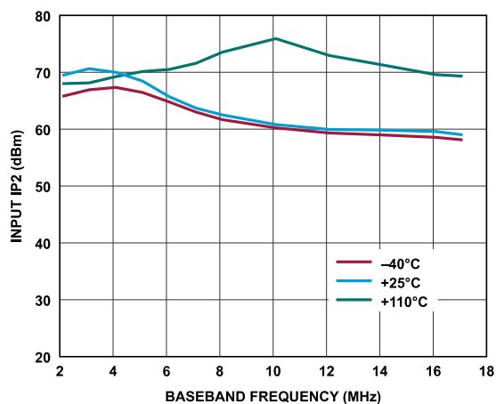
Figure 138. Receiver Input IP2 vs. Baseband Frequency, ADC = Low Power, F1 = Baseband Frequency, F2 = Baseband Frequency + 1 MHz, Gain Index = 255
