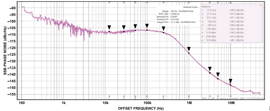
Figure 295. Internal Local Oscillator Phase Noise at 2400 MHz LO
