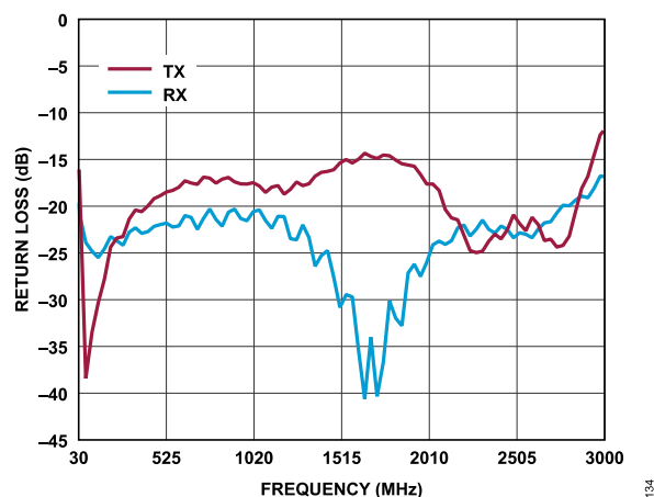
Figure 25. Receiver and Transmitter Return Loss vs. Frequency (For LO = 30 MHz to 3 GHz)
