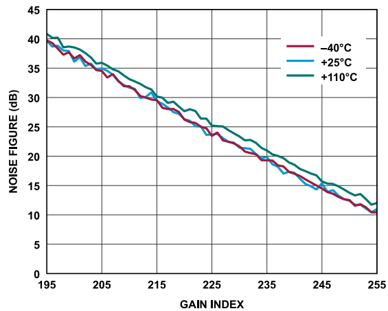
Figure 38. Receiver Noise Figure vs. Gain Index, Baseband Frequency = 5.6 MHz, ADC = High Performance
