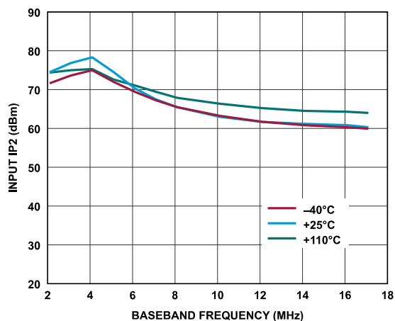
Figure 137. Receiver Input IP2 vs. Baseband Frequency, ADC = High Performance, F1 = Baseband Frequency, F2 = Baseband Frequency + 1 MHz, Gain Index = 255
