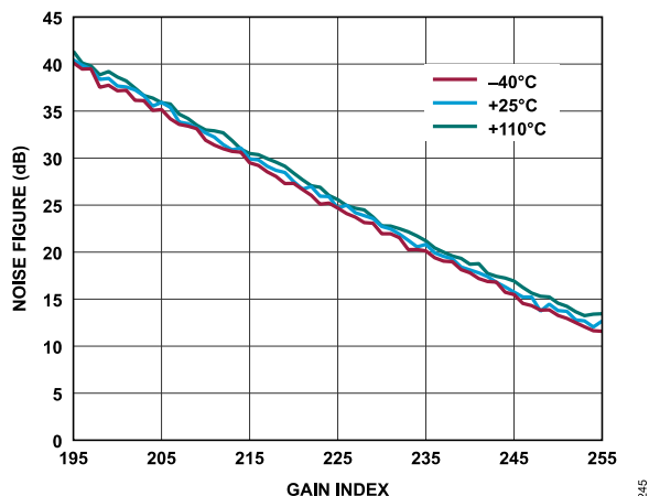
Figure 120. Receiver Noise Figure vs. Gain Index, Baseband Frequency = 5.6 MHz, ADC = High Performance
