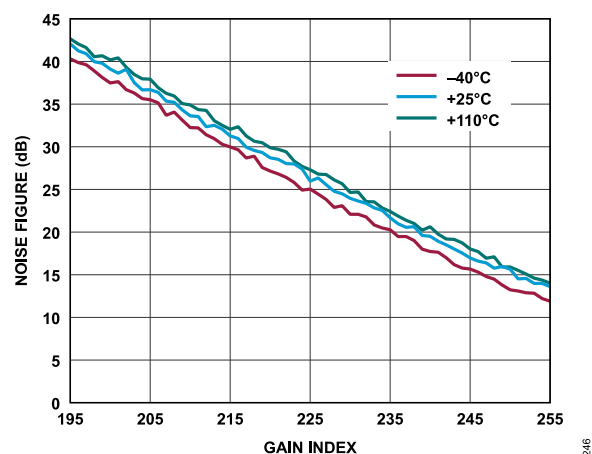
Figure 122. Receiver Noise Figure vs. Gain Index, Baseband Frequency = 5.6 MHz, ADC = Low Power
