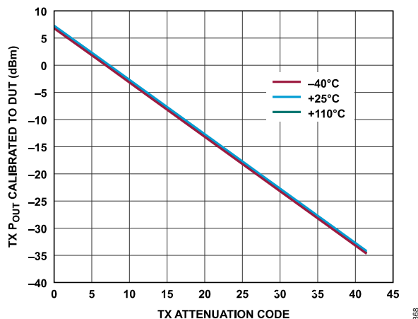
Figure 209. Transmitter Absolute Power vs. Transmitter Attenuation Code, Baseband Frequency = 2.1 kHz, Backoff = 0.2 dBFS
