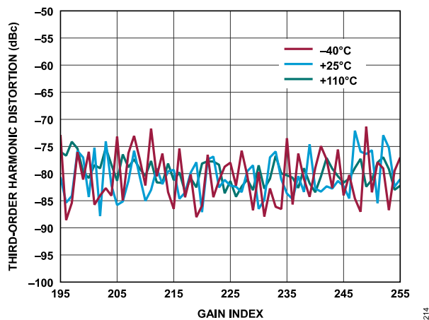
Figure 100. Receiver Third-Order Harmonic Distortion vs. Gain Index, Baseband Frequency = 5.6 MHz, ADC = Low Power
