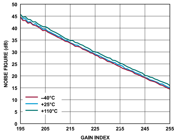
Figure 218. Receiver Noise Figure vs. Gain Index, Baseband Frequency = 2.1 kHz, ADC = Low Power
