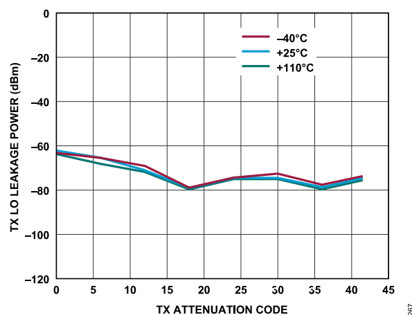
Figure 147. Transmitter LO Leakage Power vs. Transmitter Attenuation Code, Baseband Frequency = 18 MHz, Backoff = 6 dBFS, Initialization Calibration Only
