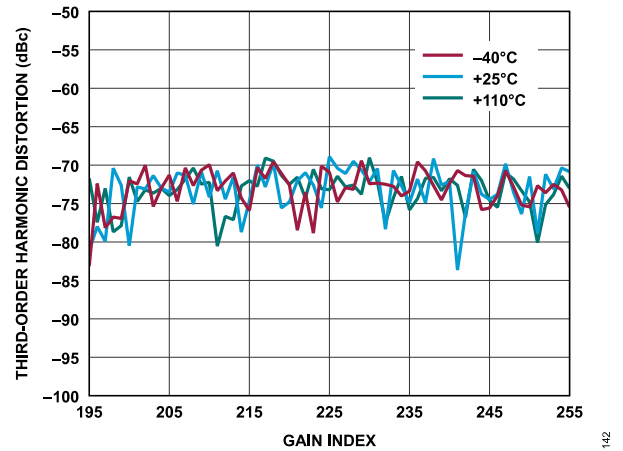
Figure 46. Receiver Third-Order Harmonic Distortion vs. Gain Index, Baseband Frequency = 5.6 MHz, ADC = Low Power
