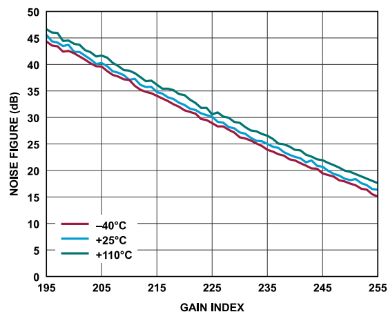
Figure 180. Receiver Noise Figure vs. Gain Index, Baseband Frequency = 2.1 kHz, ADC = Low Power
