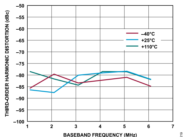
Figure 101. Receiver Third-Order Harmonic Distortion vs. Baseband Frequency, Gain Index = 255, ADC = Low Power
