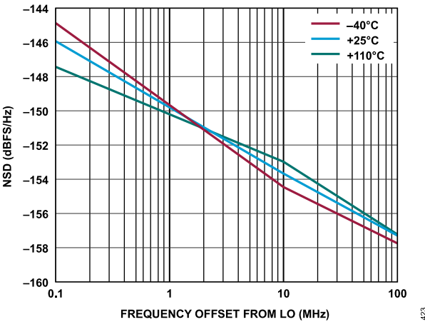
Figure 234. Transmitter NSD vs. Frequency Offset from LO, Baseband Frequency = 2.1 kHz, Transmitter Channel = Ch1
