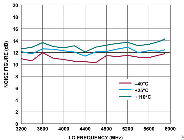
Figure 121. Receiver Noise Figure vs. LO Frequency, Baseband Frequency = 5.6 MHz, ADC = High Performance
