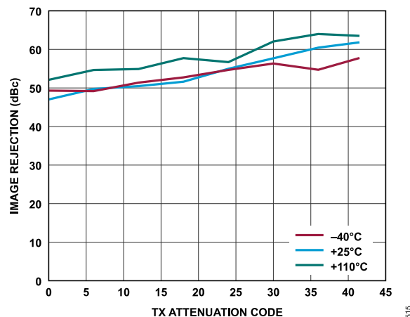
Figure 287. Transmitter Image Rejection vs. Transmitter Attenuation Code, Baseband Frequency = 2.1 kHz, Backoff = 0.2 dBFS, Initialization Calibration Only
