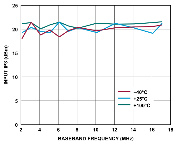
Figure 22. Receiver Input IP3 vs. Baseband Frequency, ADC = Low Power, F1 = Baseband Frequency, F2 = Baseband Frequency + 1 MHz, Gain Index = 255
