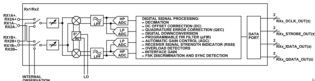
Figure 299. Receiver Architecture
