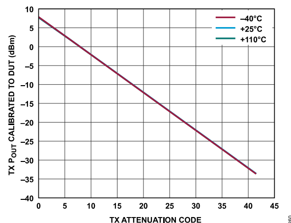
Figure 140. Transmitter Absolute Power vs. Transmitter Attenuation Code, Baseband Frequency = 18 MHz, Backoff = 0.2 dBFS
