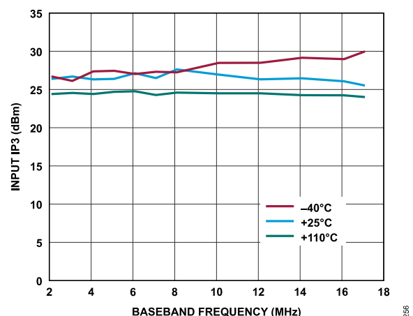
Figure 135. Receiver Input IP3 vs. Baseband Frequency, ADC = High Performance, F1 = Baseband Frequency, F2 = Baseband Frequency + 1 MHz, Gain Index = 255
