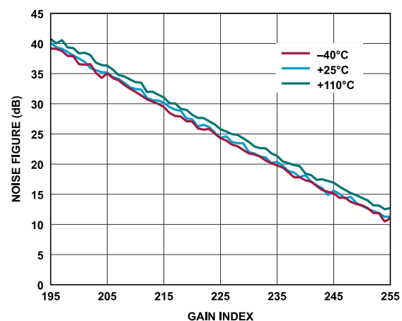
Figure 92. Receiver Noise Figure vs. Gain Index, Baseband Frequency = 5.6 MHz, ADC = High Performance
