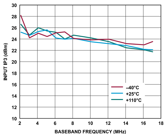
Figure 50. Receiver Input IP3 vs. Baseband Frequency, ADC = Low Power, F1 = Baseband Frequency, F2 = Baseband Frequency + 1 MHz, Gain Index = 255
