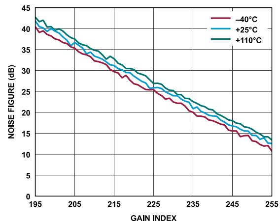
Figure 93. Receiver Noise Figure vs. Gain Index, Baseband Frequency = 5.6 MHz, ADC = Low Power
