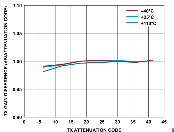
Figure 229. Transmitter Attenuation Delta (Error) vs. Transmitter Attenuation Code, Baseband Frequency = 2.1 kHz, Backoff = 0.2 dBFS
