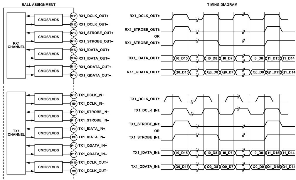
Figure 303. LSSI in 2-Lane Data Mode, DDR
