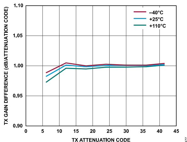
Figure 267. Transmitter Attenuation Delta (Error) vs. Transmitter Attenuation Code, Baseband Frequency = 2.1 kHz, Backoff = 0.2 dBFS
