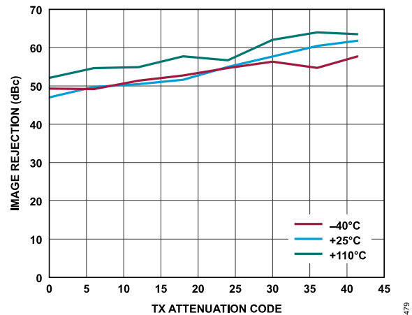
Figure 268. Transmitter Image Rejection vs. Transmitter Attenuation Code, Baseband Frequency = 2.1 kHz, Backoff = 0.2 dBFS, Initialization Calibration Only
