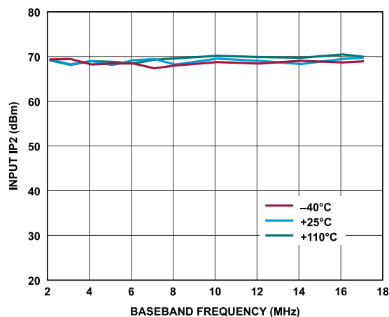
Figure 24. Receiver Input IP2 vs. Baseband Frequency, ADC = Low Power, F1 = Baseband Frequency, F2 = Baseband Frequency + 1 MHz, Gain Index = 255
