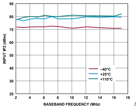
Figure 23. Receiver Input IP2 vs. Baseband Frequency, ADC = High Performance, F1 = Baseband Frequency, F2 = Baseband Frequency + 1 MHz, Gain Index = 255
