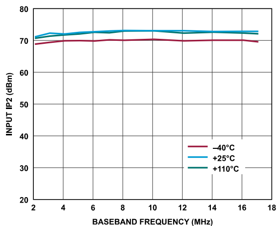
Figure 105. Receiver Input IP2 vs. Baseband Frequency, ADC = High Performance, F1 = Baseband Frequency, F2 = Baseband Frequency + 1 MHz, Gain Index = 255
