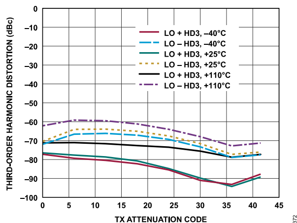
Figure 212. Transmitter Third-Order Harmonic Distortion vs. Transmitter Attenuation Code, Baseband Frequency = 2.1 kHz, Backoff = 0.2 dBFS
