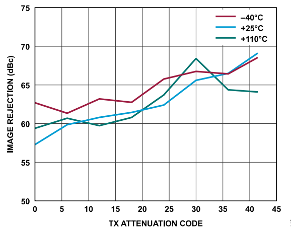
Figure 249. Transmitter Image Rejection vs. Transmitter Attenuation Code, Baseband Frequency = 2.1 kHz, Backoff = 0.2 dBFS, Initialization Calibration Only
