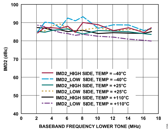
Figure 34. Transmitter Second-Order Intermodulation Distortion (IMD2) vs. Baseband Frequency, Transmitter Attenuation Code = 0, F1 = Baseband Frequency, F2 = Baseband Frequency + 1 MHz
