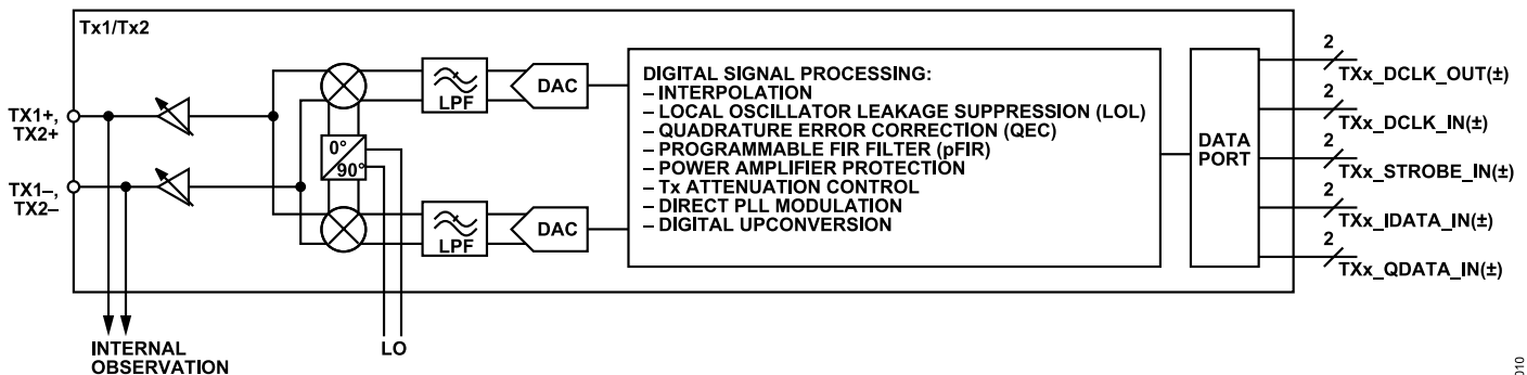
Figure 298. Transmitter Architecture
