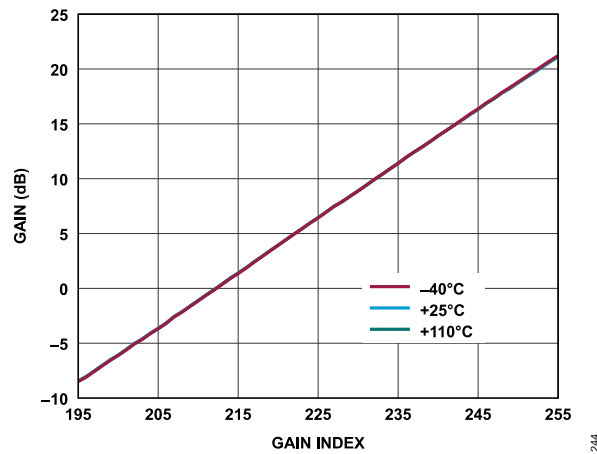
Figure 118. Receiver Absolute Gain (Complex) vs. Gain Index, Baseband Frequency = 5.6 MHz, ADC = High Performance, P_{OUT} = -9.6 dBFS
