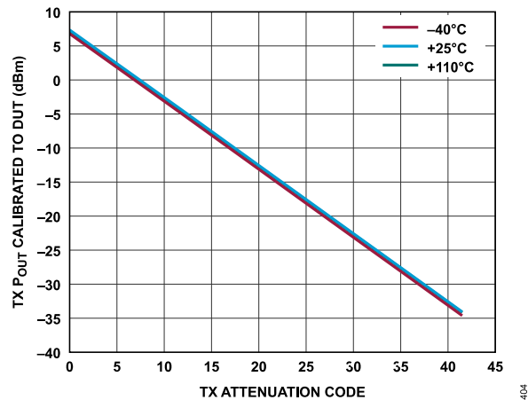
Figure 228. Transmitter Absolute Power vs. Transmitter Attenuation Code, Baseband Frequency = 2.1 kHz, Backoff = 0.2 dBFS
