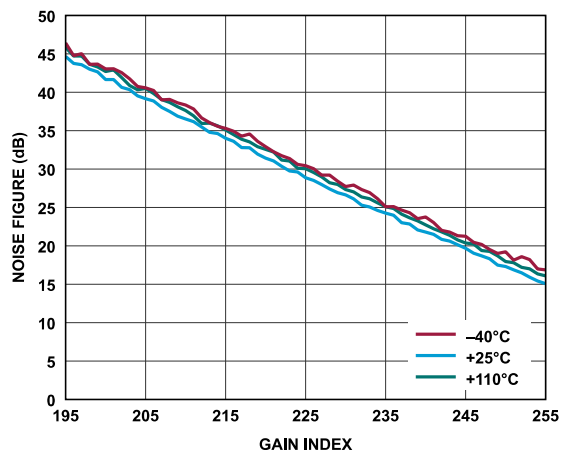
Figure 199. Receiver Noise Figure vs. Gain Index, Baseband Frequency = 2.1 kHz, ADC = Low Power
