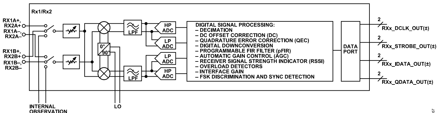
Figure 299. Receiver Architecture
