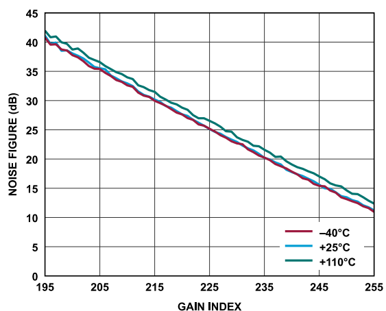
Figure 198. Receiver Noise Figure vs. Gain Index, Baseband Frequency = 2.1 kHz, ADC = High Performance
