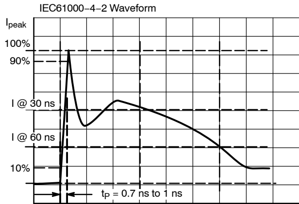
Figure 26. IEC61000-4-2 Spec
