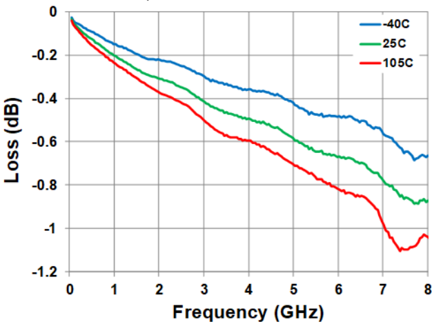
Figure 36. EVKIT Trace and Connector Loss vs. Temperature
