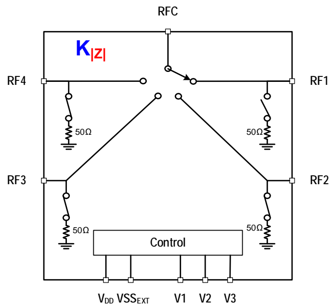
Figure 1. Block Diagram
