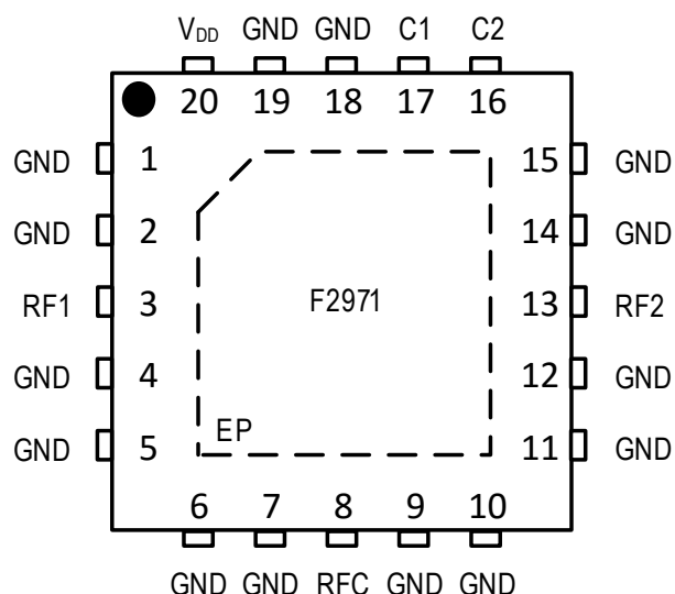
Figure 2. Pin Assignments for 4mm x 4mm x 0.75mm 20-pin LQFN, NCG20P1 – Top View
