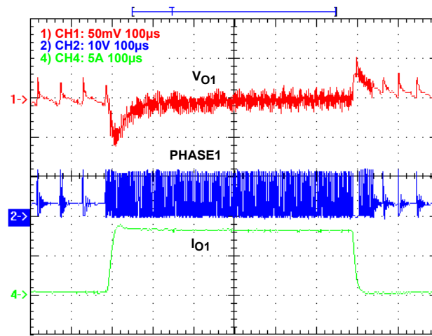
FIGURE 14. TRANSIENT RESPONSE, V_{IN} = 12V , V_{O1} = 3.3V , I_{O1} = 0.1A/8.1A @ 2.5A/\mu s
