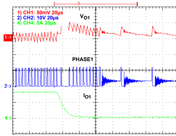
FIGURE 16. LOAD RELEASE RESPONSE, V_{IN} = 12V , V_{O1} = 3.3V , I_{O1} = 0.1A/8.1A @ 2.5A/\mu s
