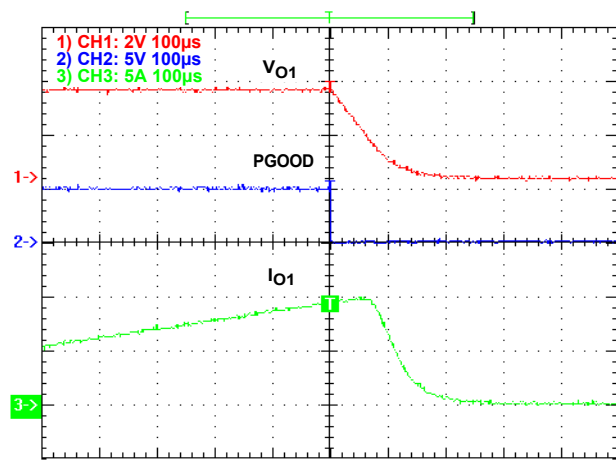
FIGURE 20. OVERCURRENT PROTECTION, V_{IN} = 12V , V_{O1} = 3.3V
