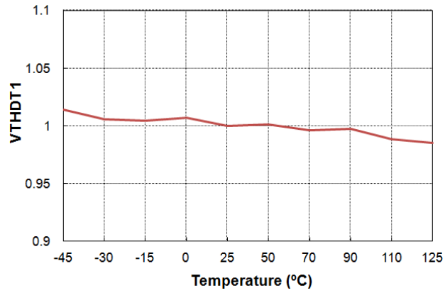
Figure 27. V THDT1 vs. Temperature
