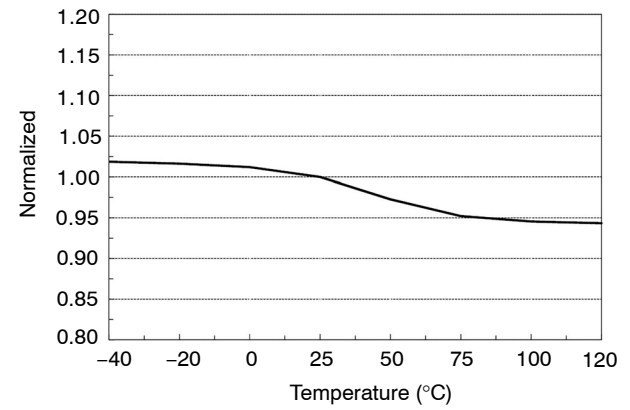
Figure 7. HV CC Stop Voltage vs. Temperature
