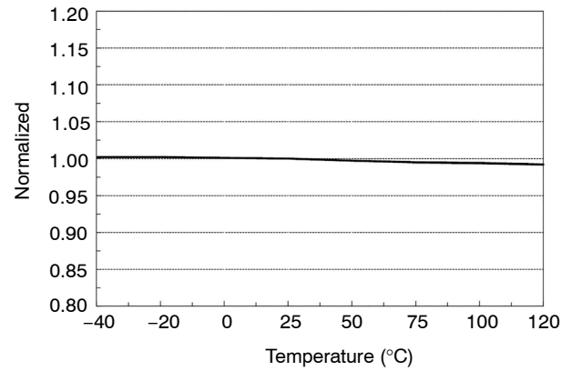
Figure 5. LV CC Stop Voltage vs. Temperature
