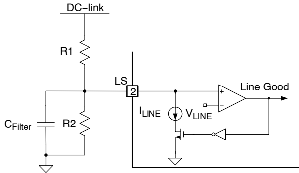
Figure 39. Line-UVLO
