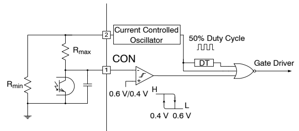
Figure 42. Pulse-Skipping Circuit
