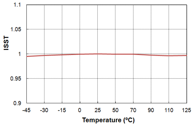
Figure 29. I SS,T vs. Temperature
