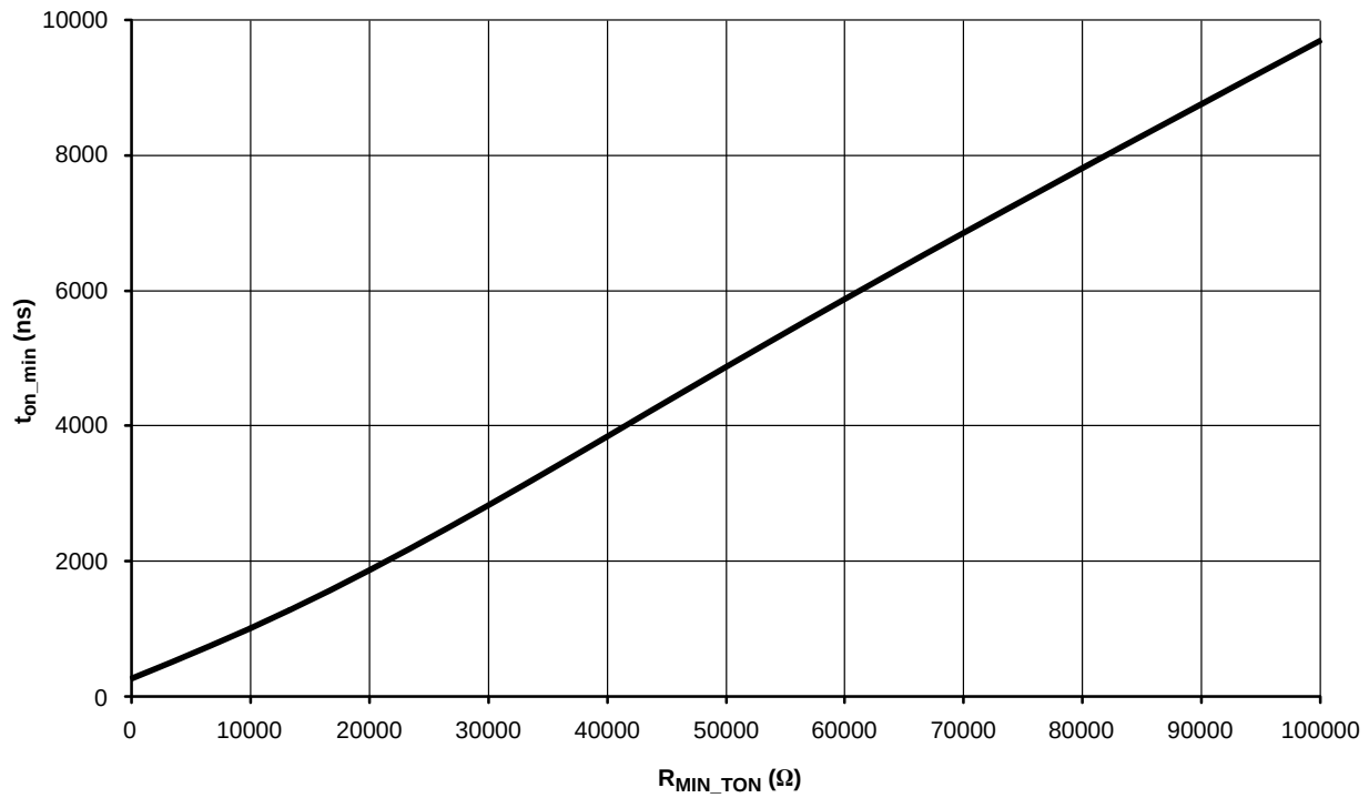
Figure 4. t_{on\_min} on R_{MIN\_TON} Dependency
