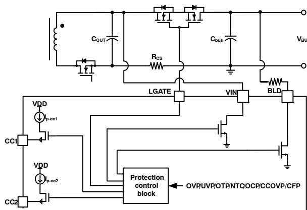
Figure 33. Protection Block Diagram
