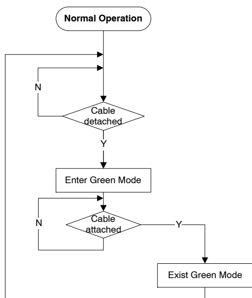
Figure 32. Green Mode Operation
