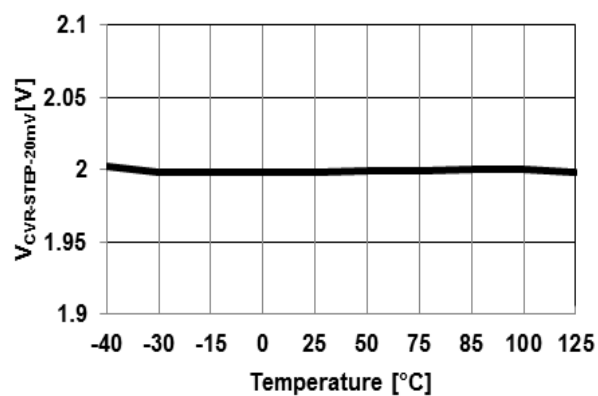
Figure 9. V_{CVR-STEP-20mV} vs. Temperature
