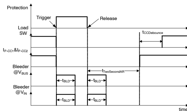
Figure 34. Auto Restart Mode Operation
