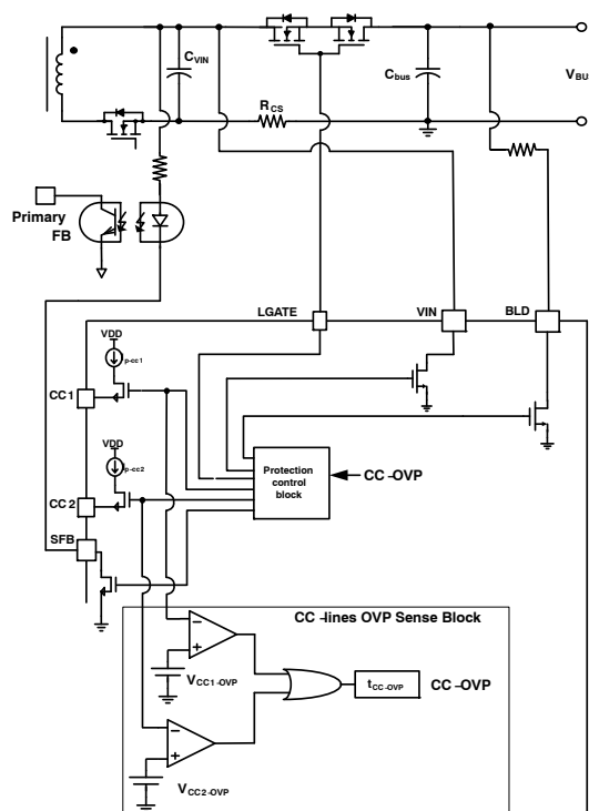
Figure 40. CC OVP Sensing Block Diagram
