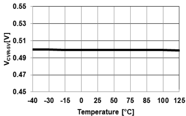
Figure 5. V_{CVR-5V} vs. Temperature
