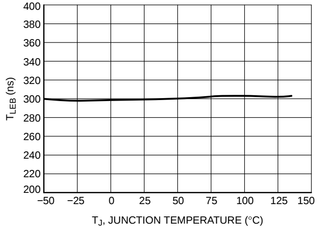
Figure 14. Leading Edge Blanking vs. Temperature
