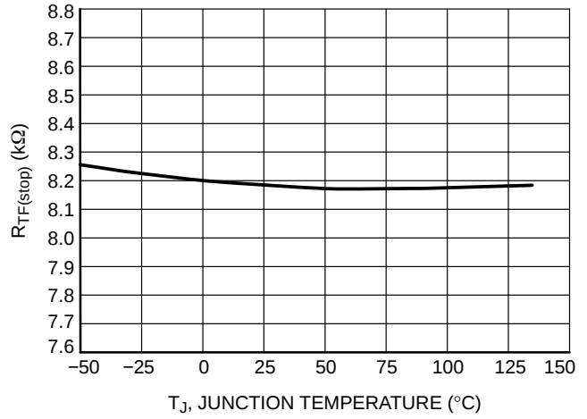
Figure 50. R TF(stop) vs. Temperature
