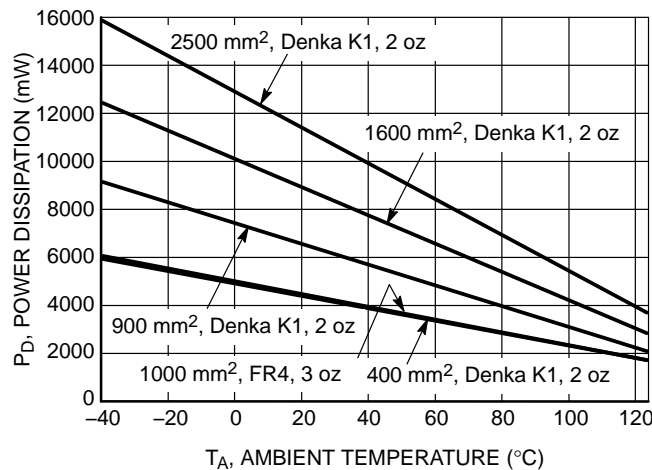
Figure 6. Power Dissipation vs. Ambient Temperature @ T_J = 175°C
