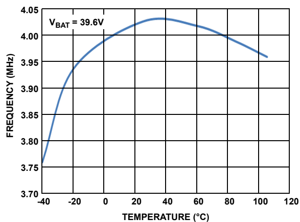
Figure 20. 4MHz Oscillator Frequency vs. Temperature
