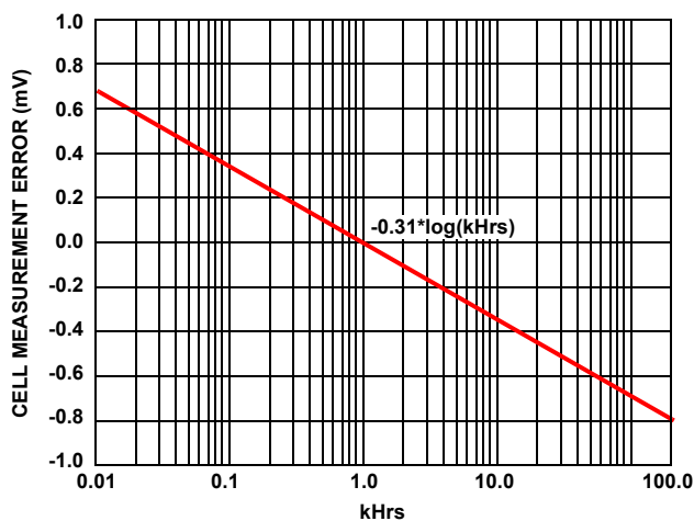
Figure 37. Long Term Drift
