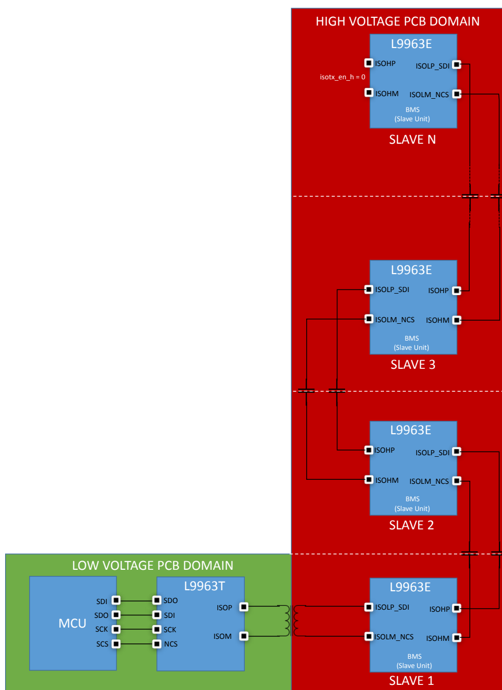
Figure 50. Centralized BMS
