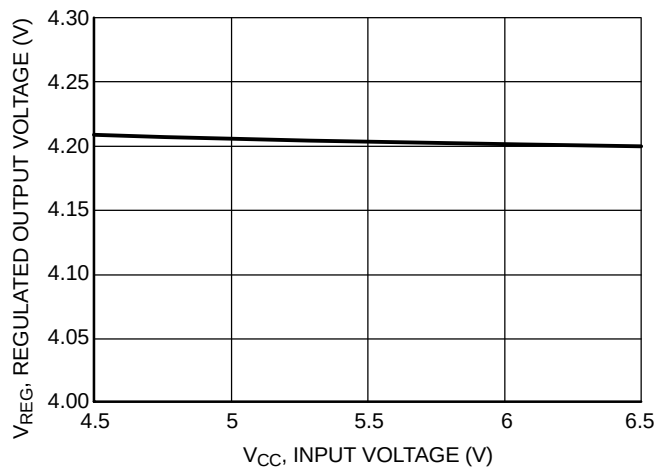
Figure 4. Regulated Output Voltage (floating) vs. Input Voltage
