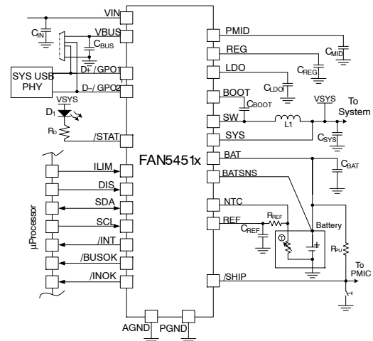
Figure 1. Typical Application
