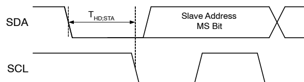
Figure 50. Start Bit
