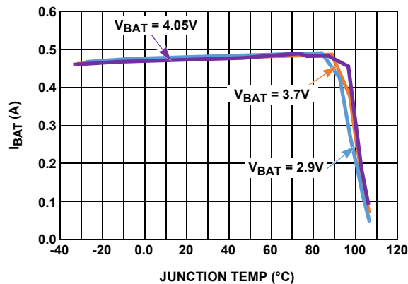
FIGURE 8. CHARGE CURRENT vs JUNCTION TEMPERATURE, R_{\text{IREF}} = 158\text{k}
