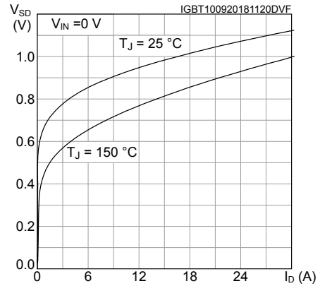
Figure 10. Diode V_{SD} vs drain current
