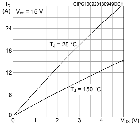
Figure 9. Output characteristics
