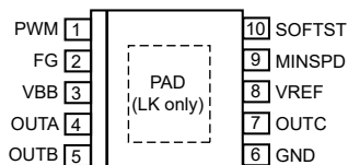
10-lead SOIC Pinout (suffix LK/LN)
