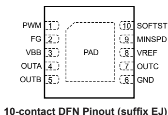
10-contact DFN Pinout (suffix EJ)
