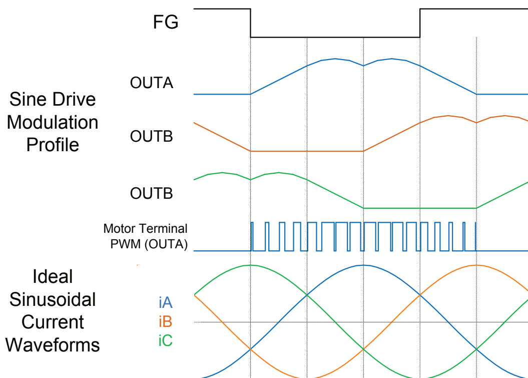
Figure 1. Sinusoidal PWM
