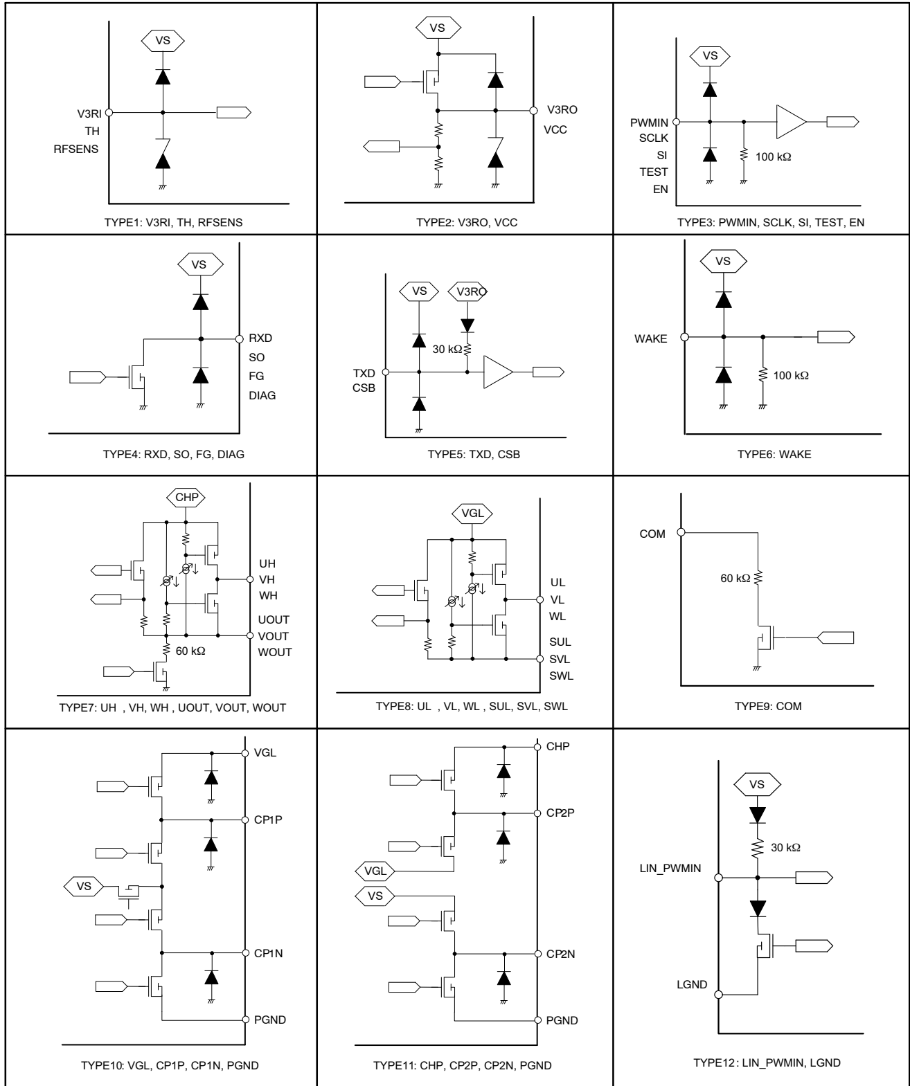
Figure 5. Pin Circuit
