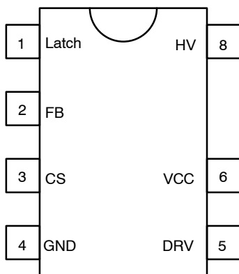
Figure 1. Pinout
