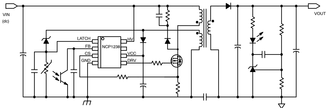
Figure 2. Typical Application
