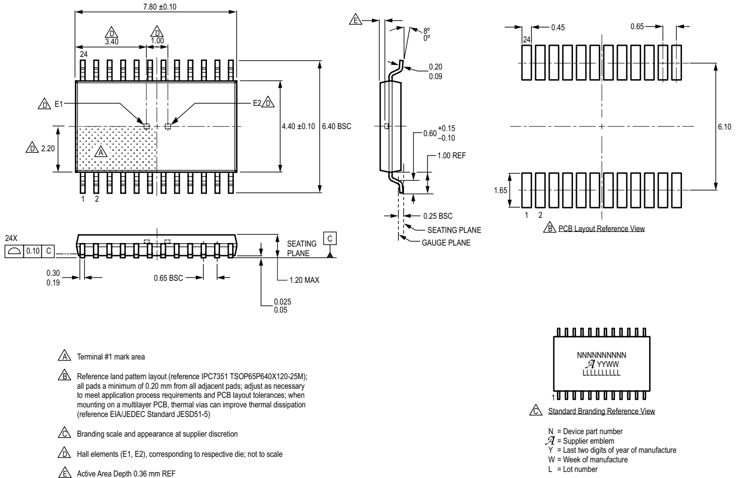
Figure 31: Package LE, 24-Pin TSSOP
